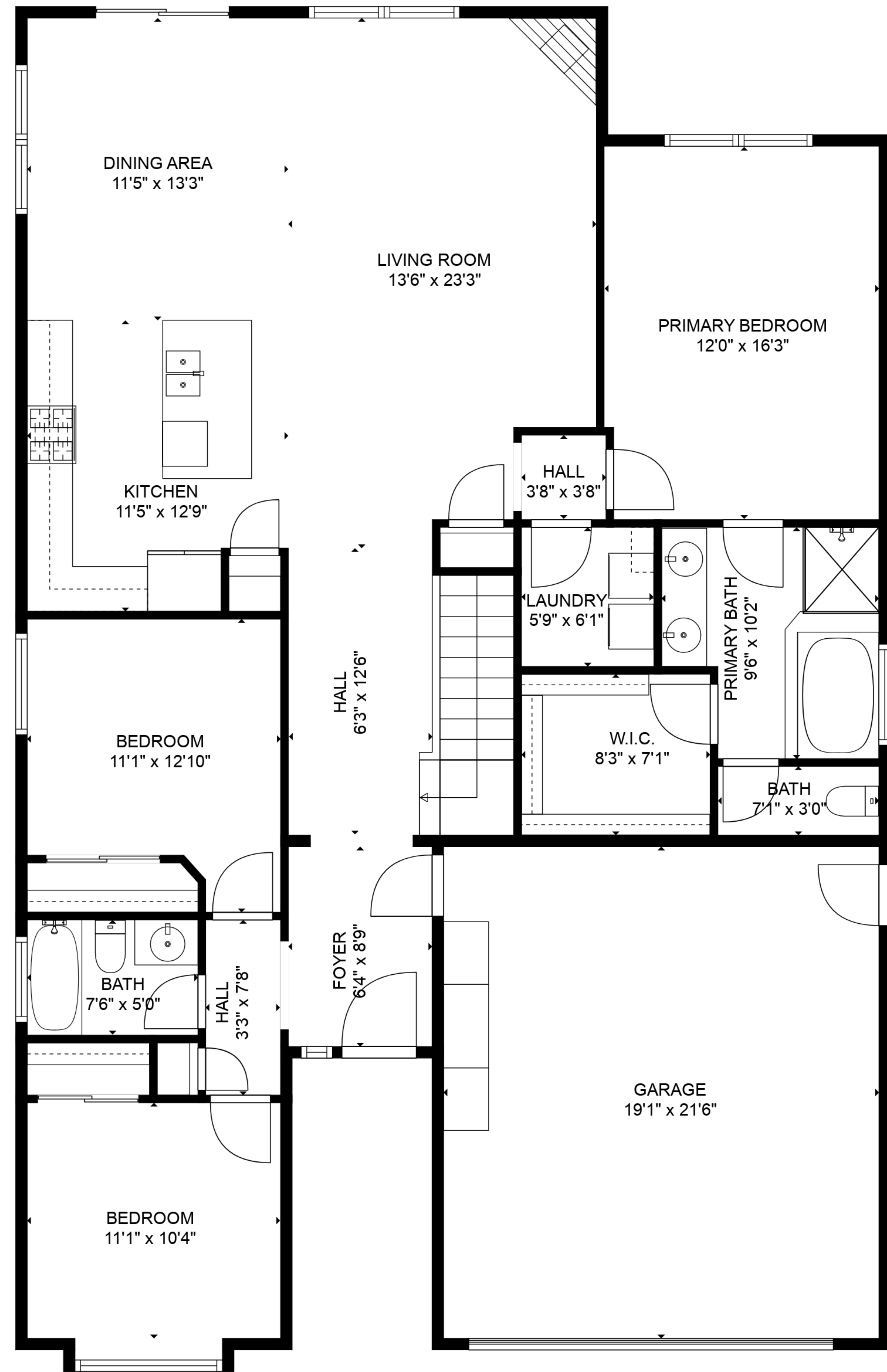
FLOOR 2
