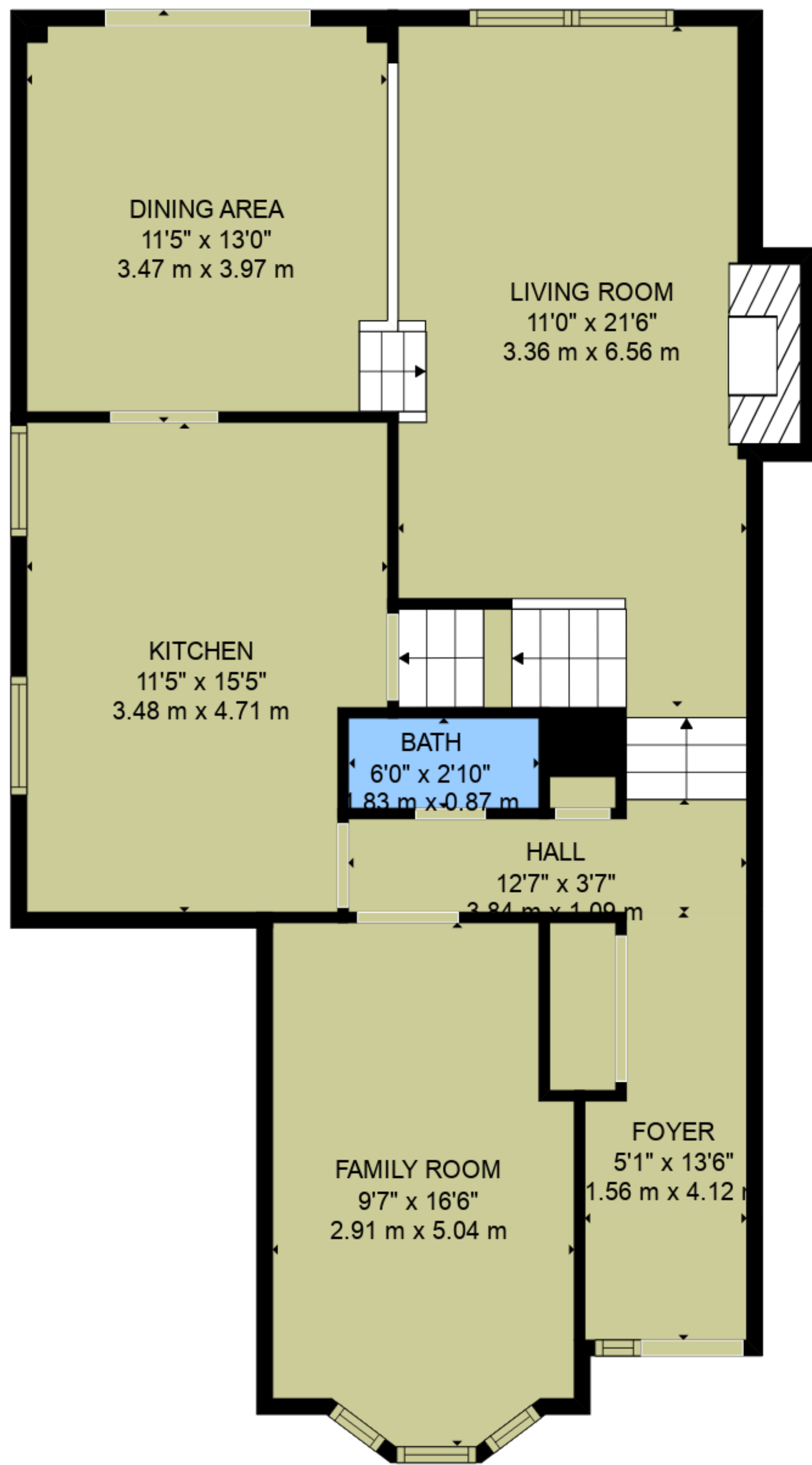
FLOOR 3
