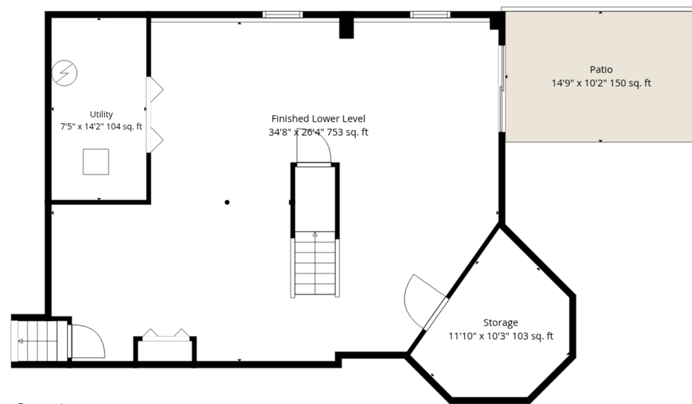
Basement
