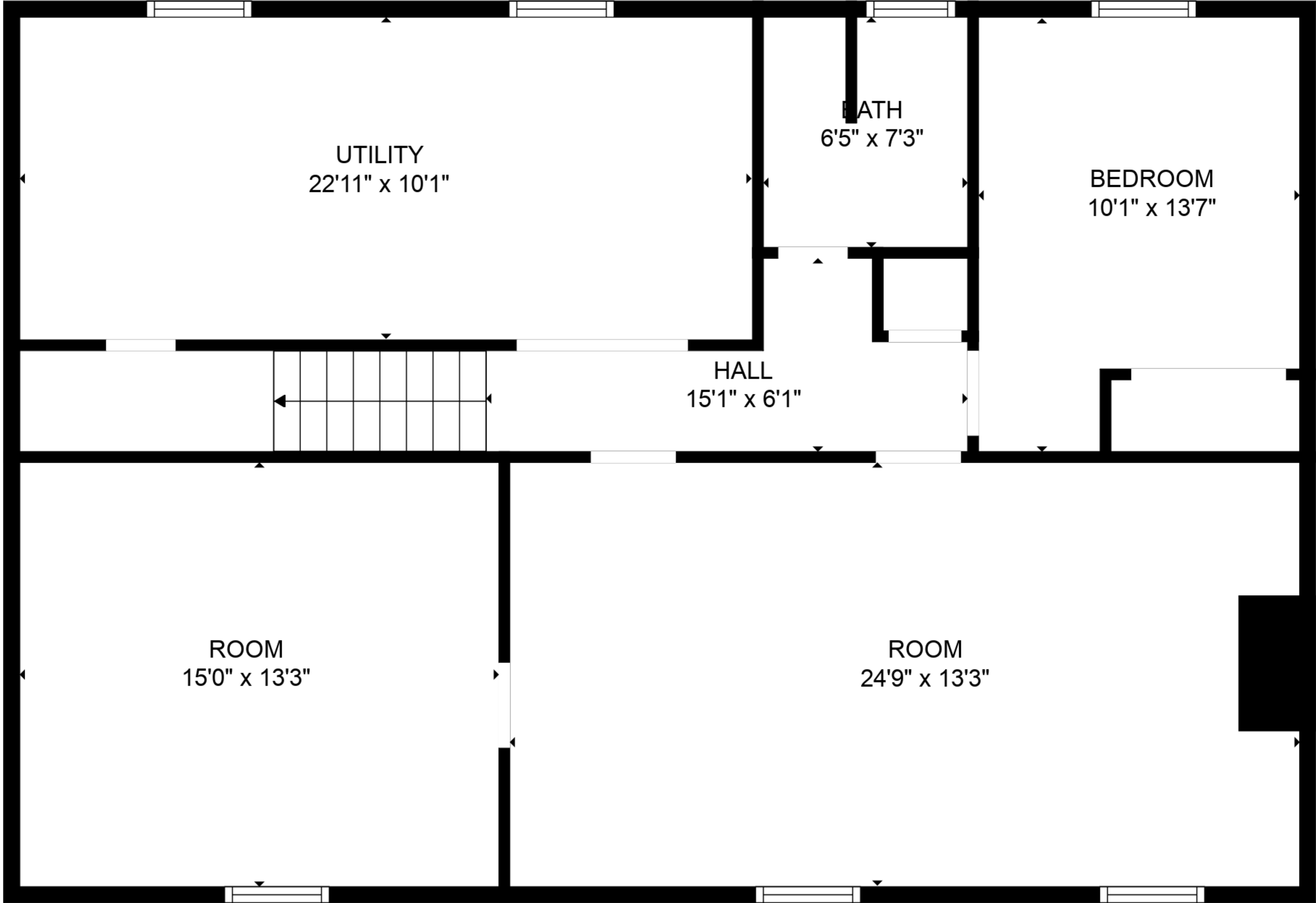
FLOOR 1
