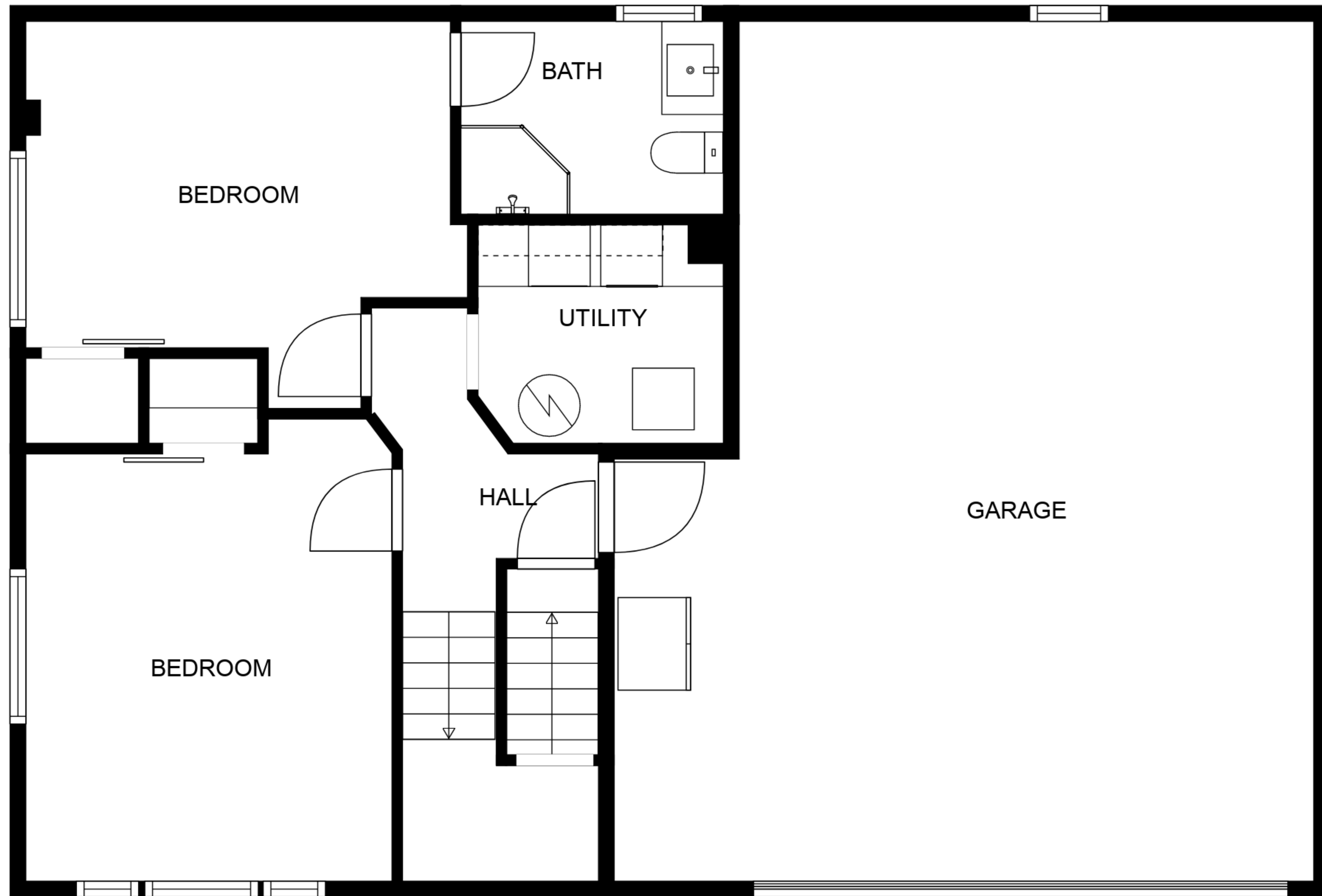
FLOOR 1
