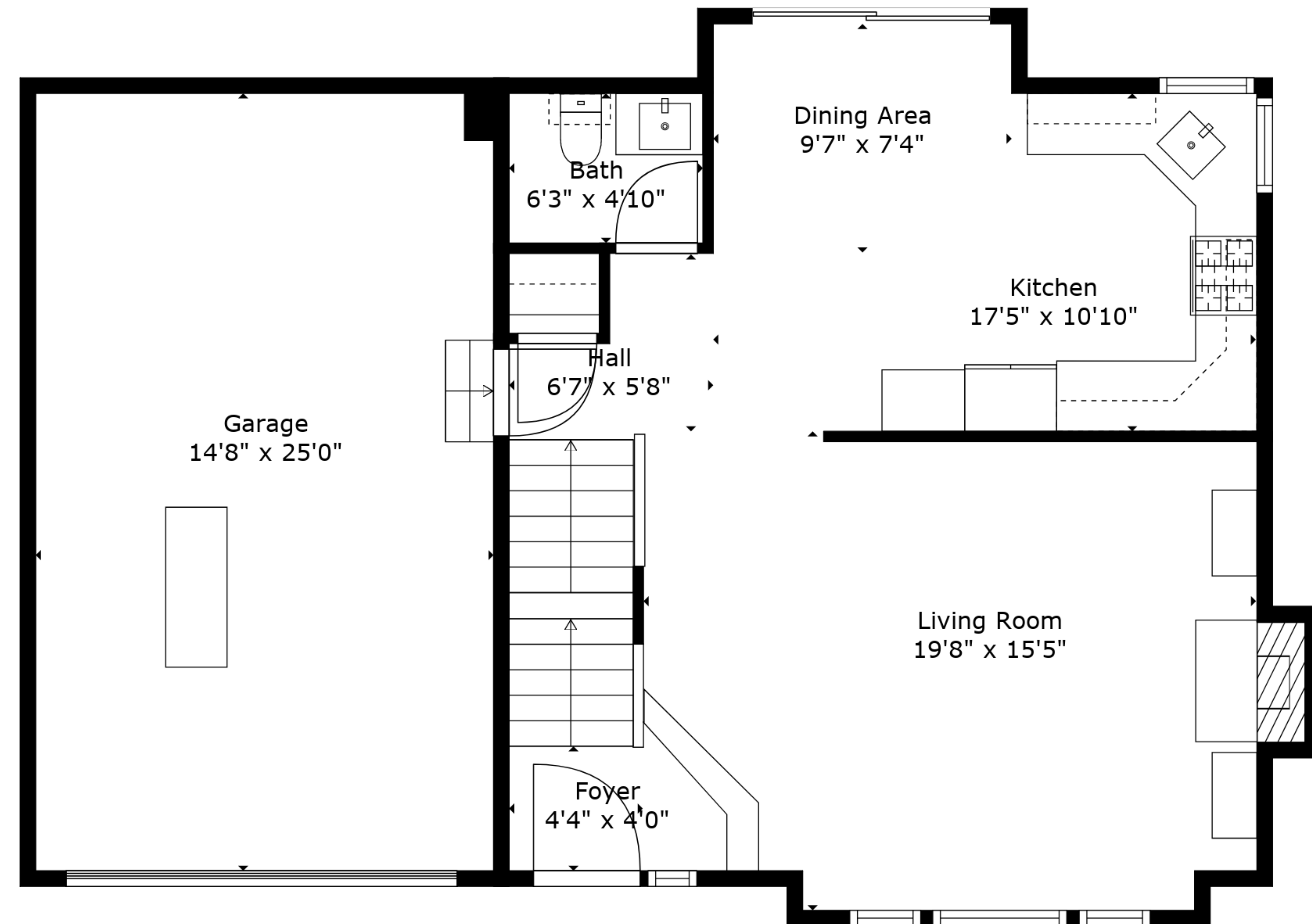
Floor 2
