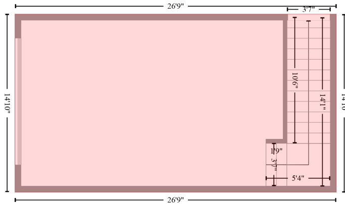
GARAGE (1) [AREA: 396]
