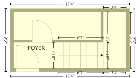
FLOOR 1 [AREA: 161]
