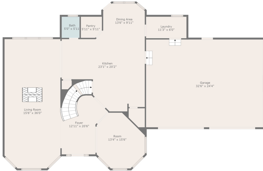
Floor 2
