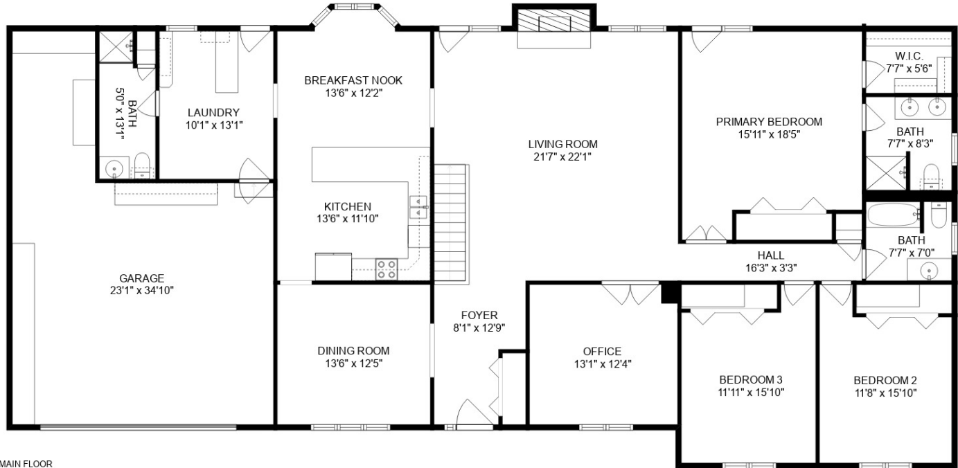
MAIN FLOOR
