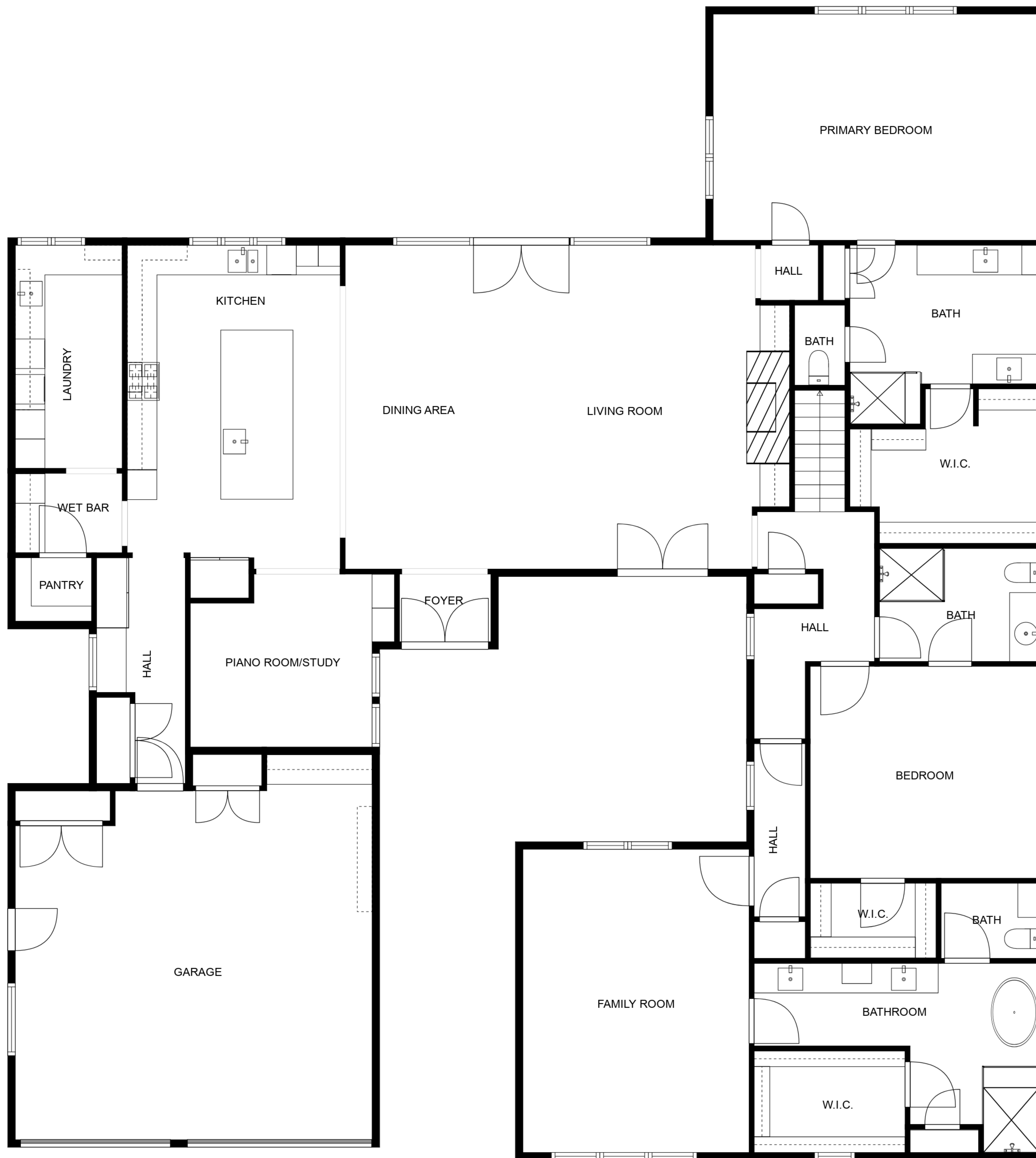
FLOOR 1
