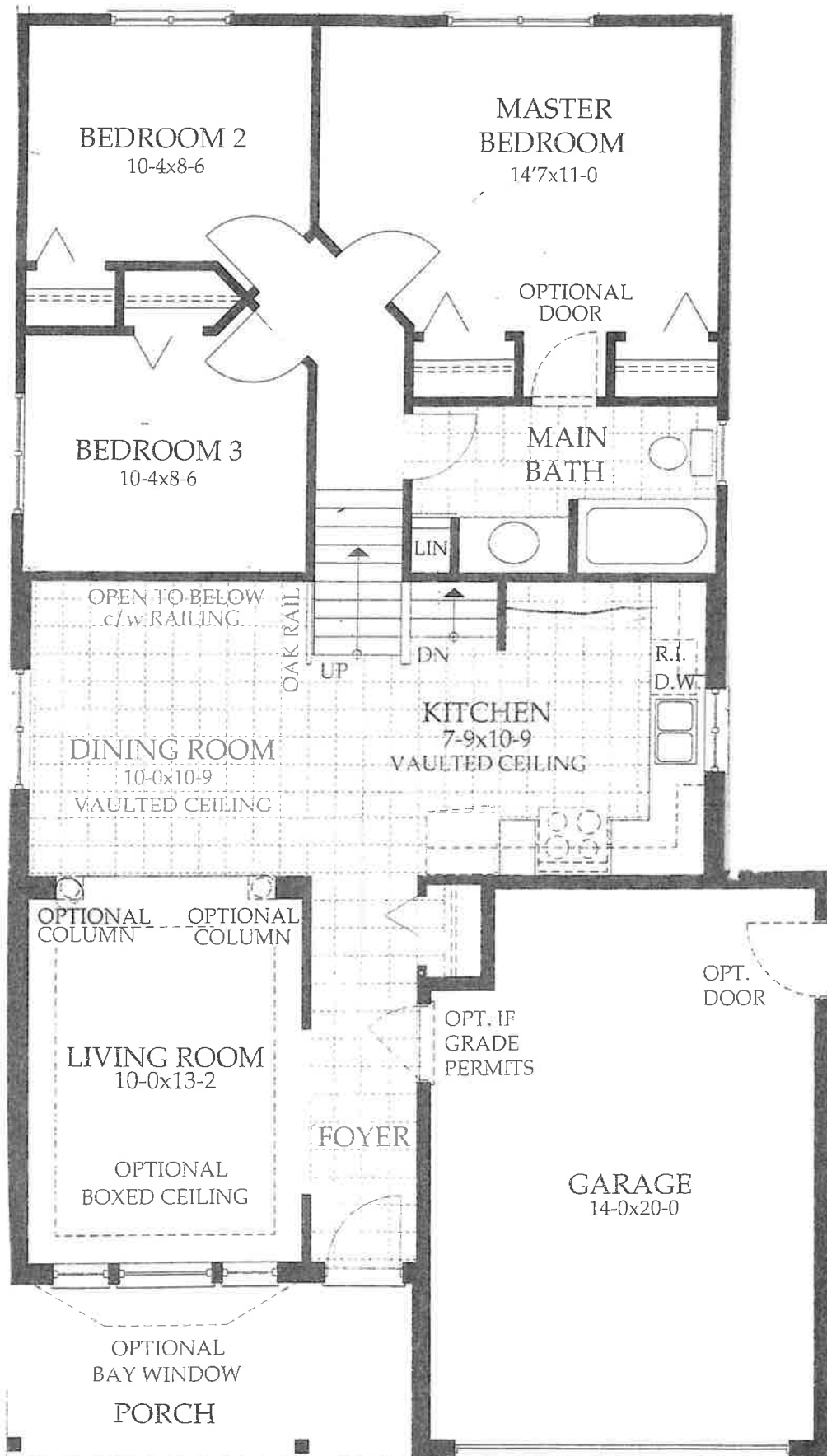
MAIN AND UPPER LEVEL FLOOR PLAN
