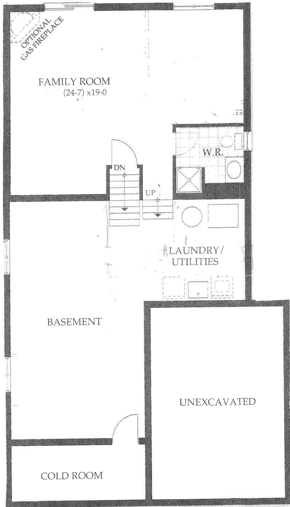
LOWER LEVEL AND BASEMENT FLOOR PLAN
