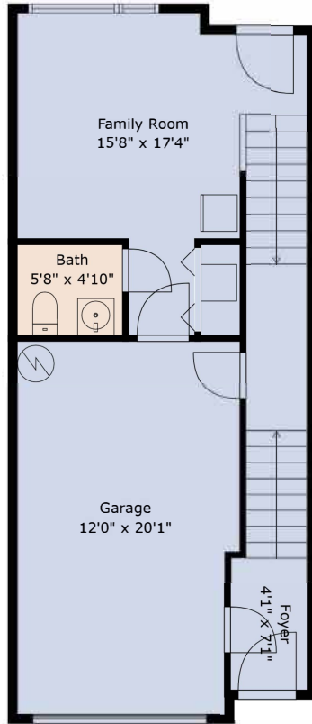
Floor 1
