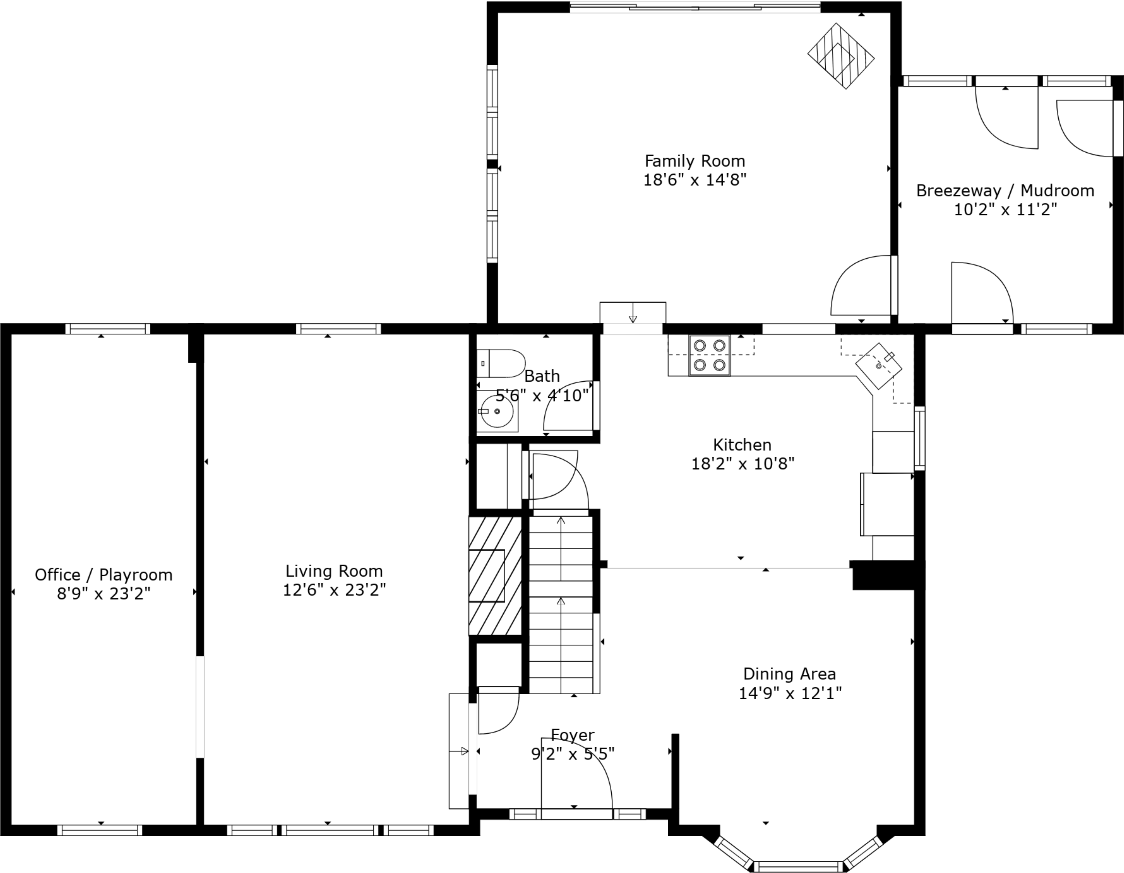
Floor 2
