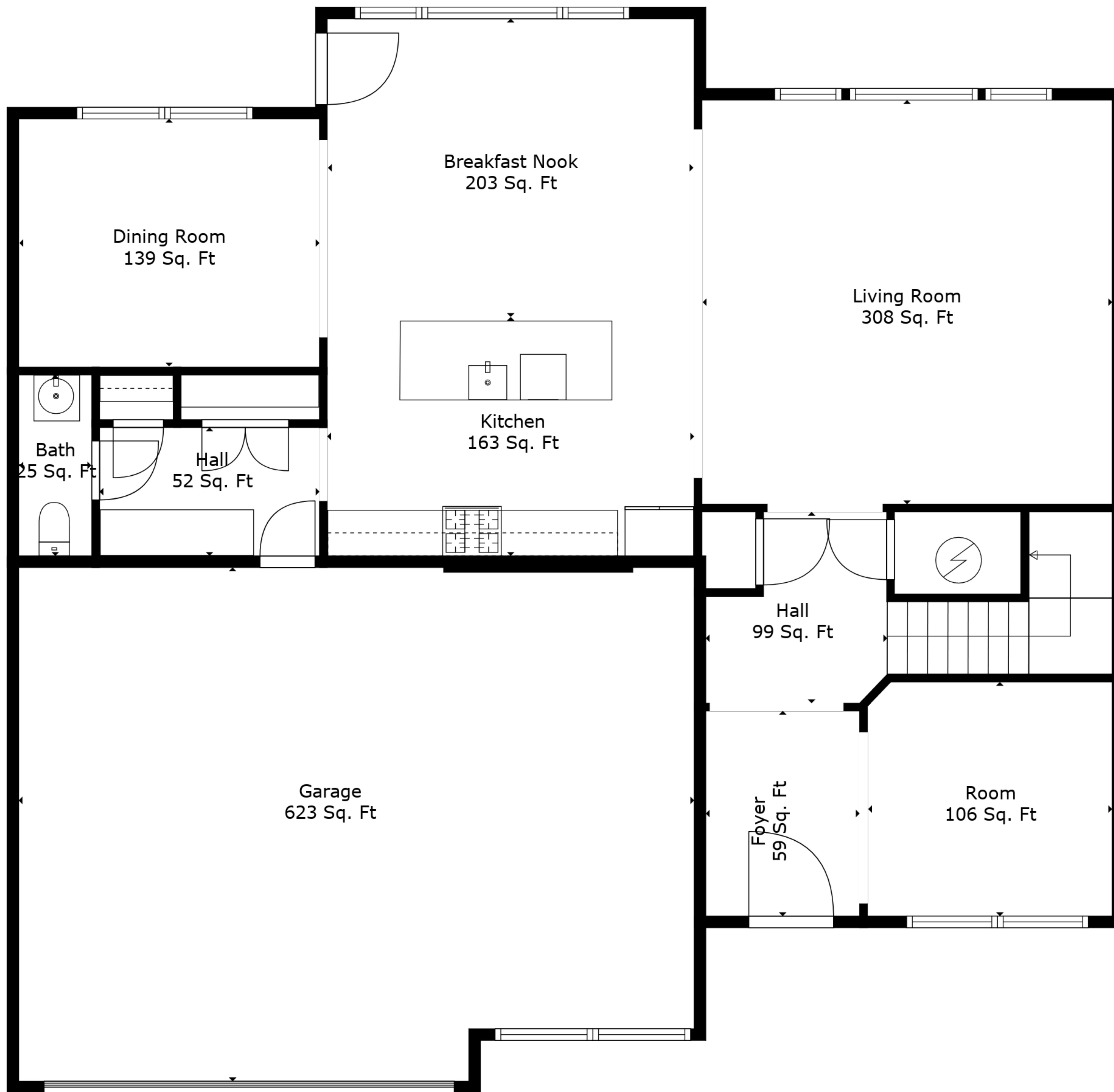
Floor 1
