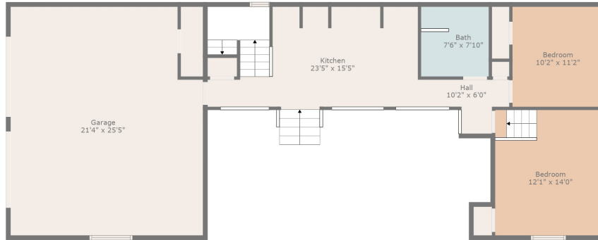
Floor 2
