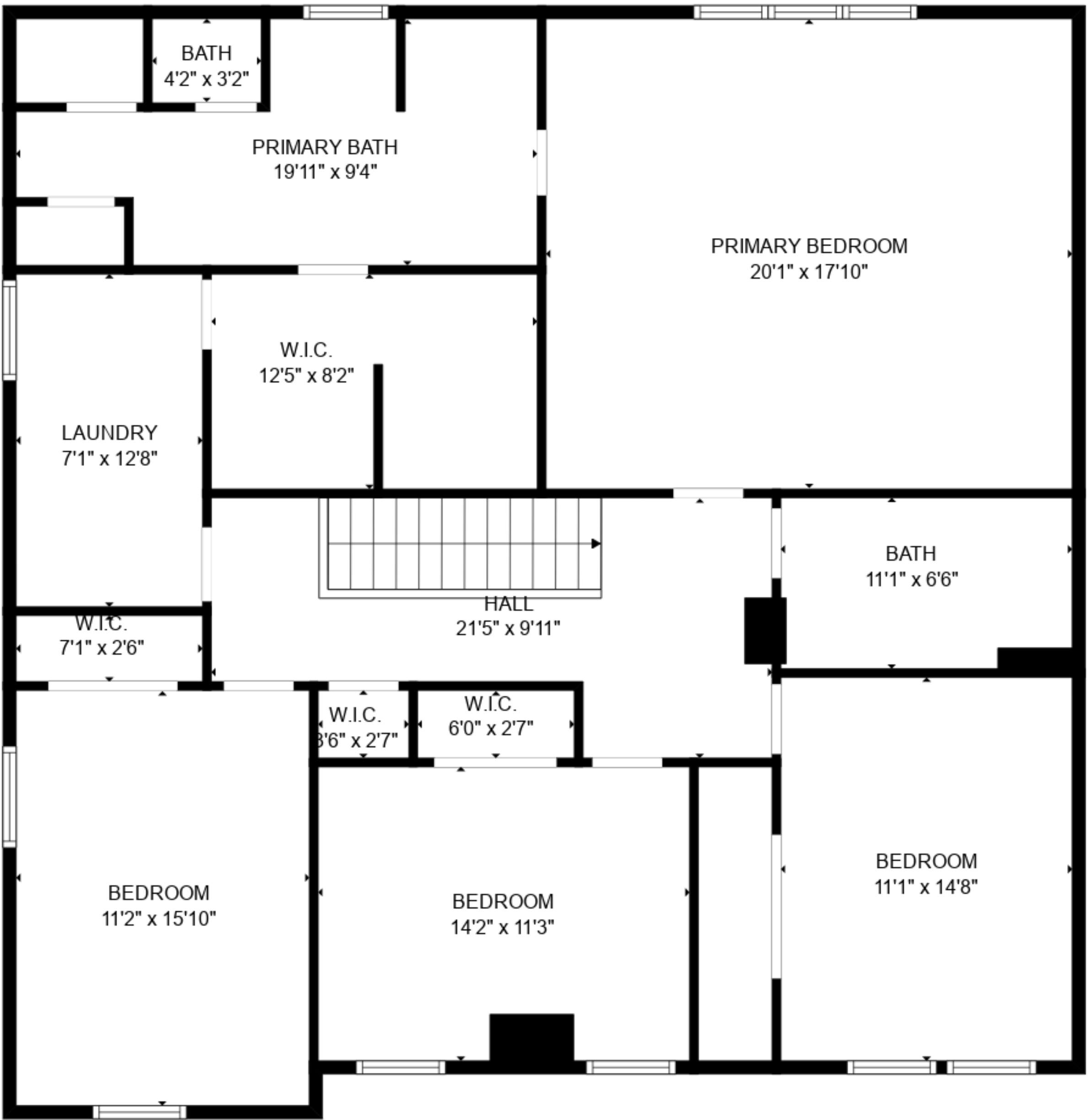
FLOOR 3
