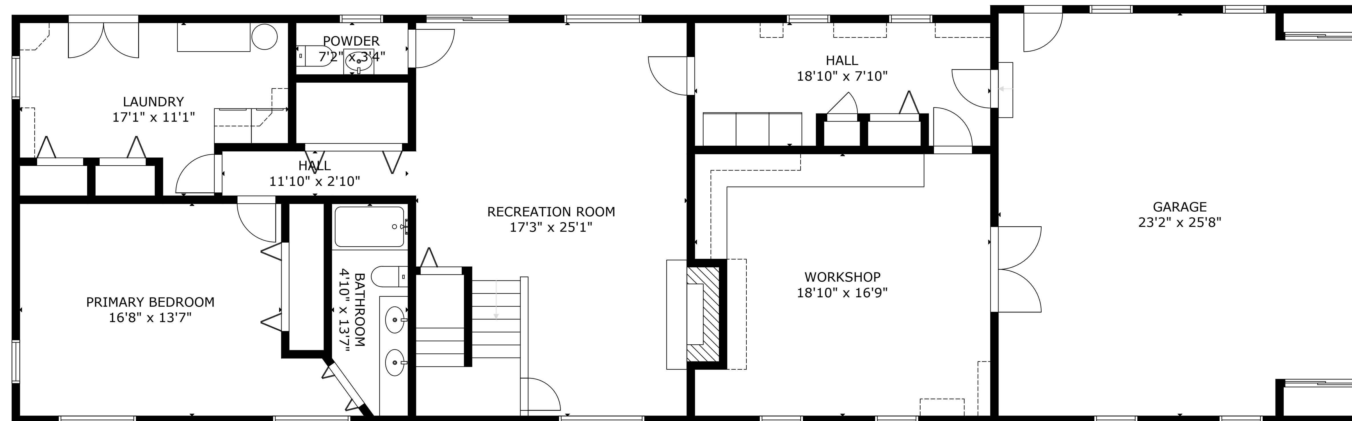
LOWER FLOOR
