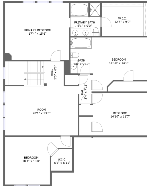
FLOOR 2
