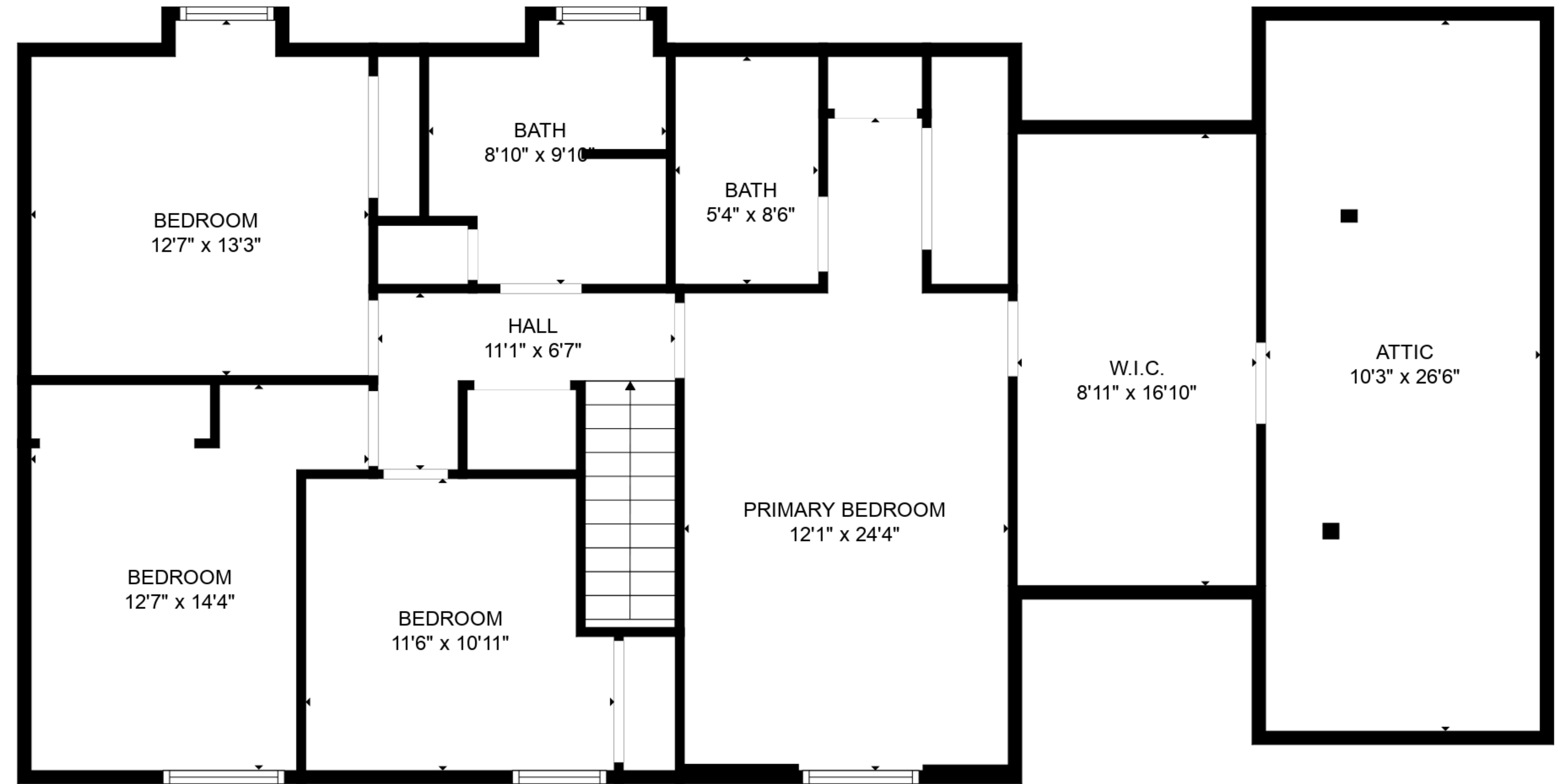
FLOOR 3
