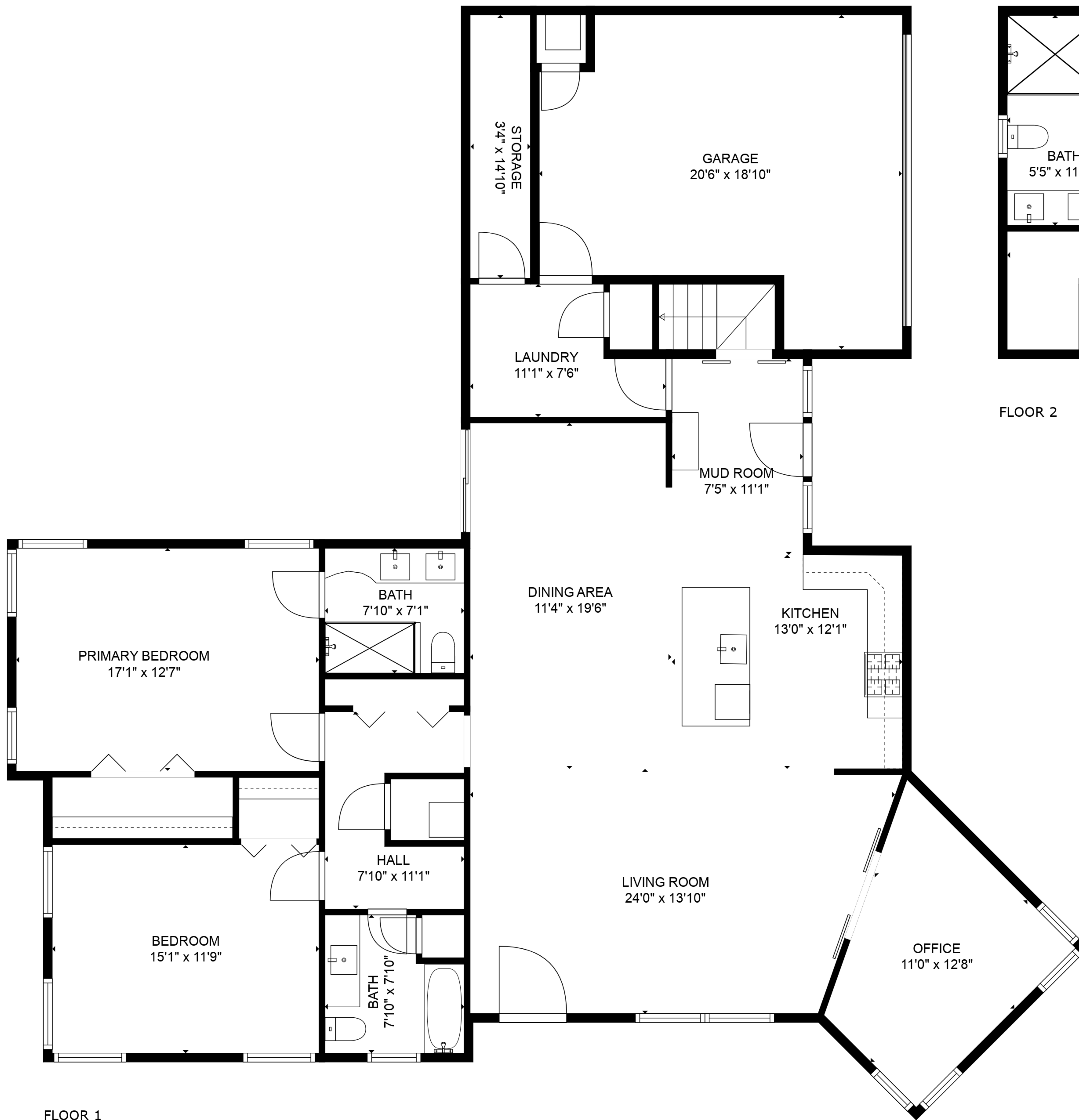
FLOOR 1
