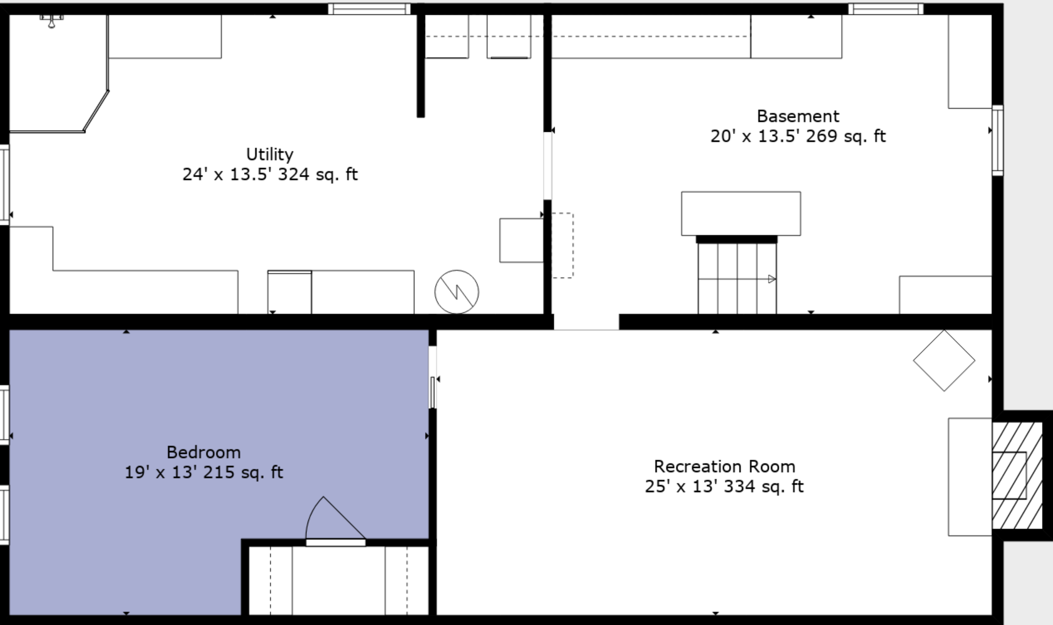
Floor 1
