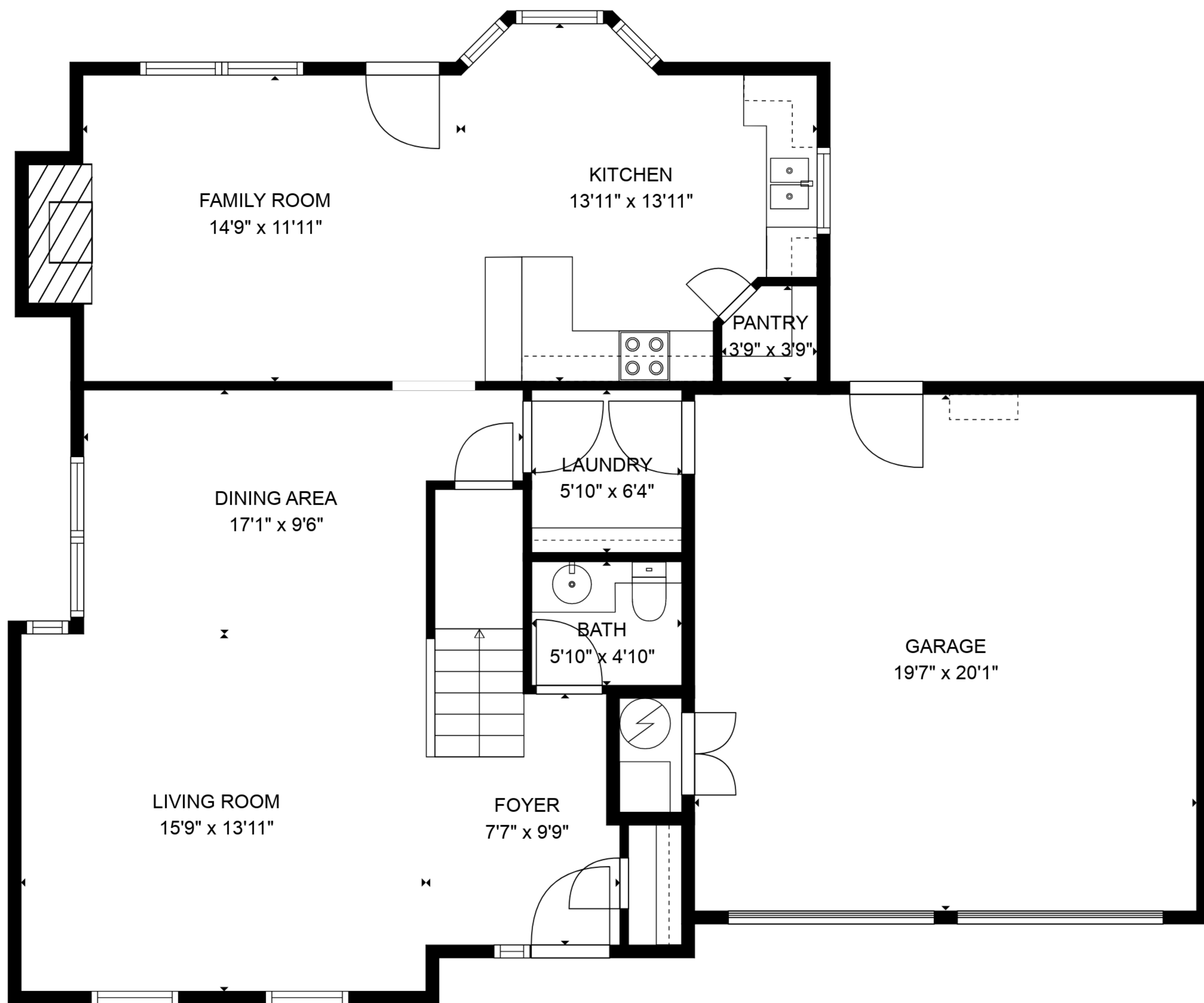
FLOOR 1
