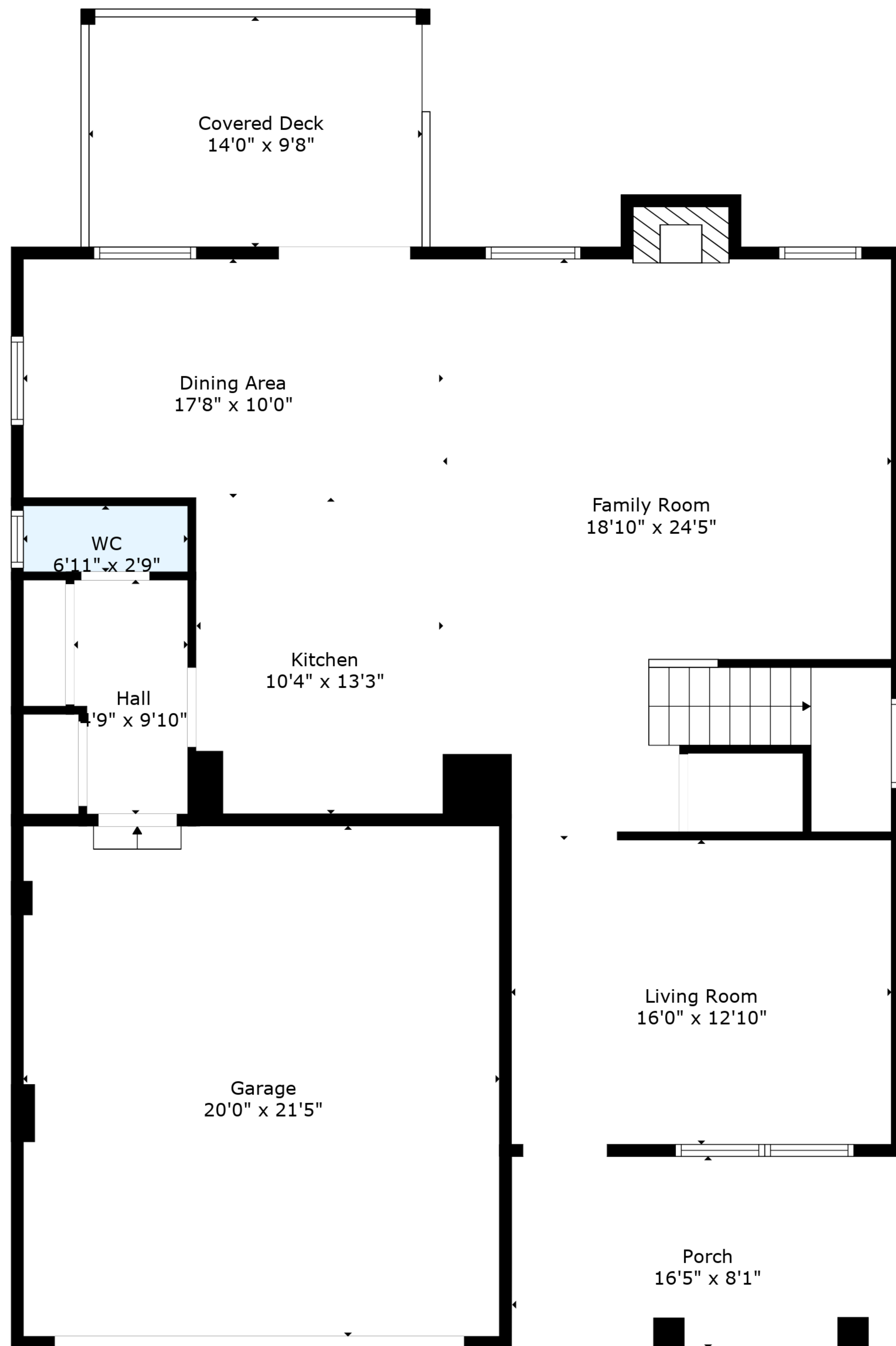
Floor 1
