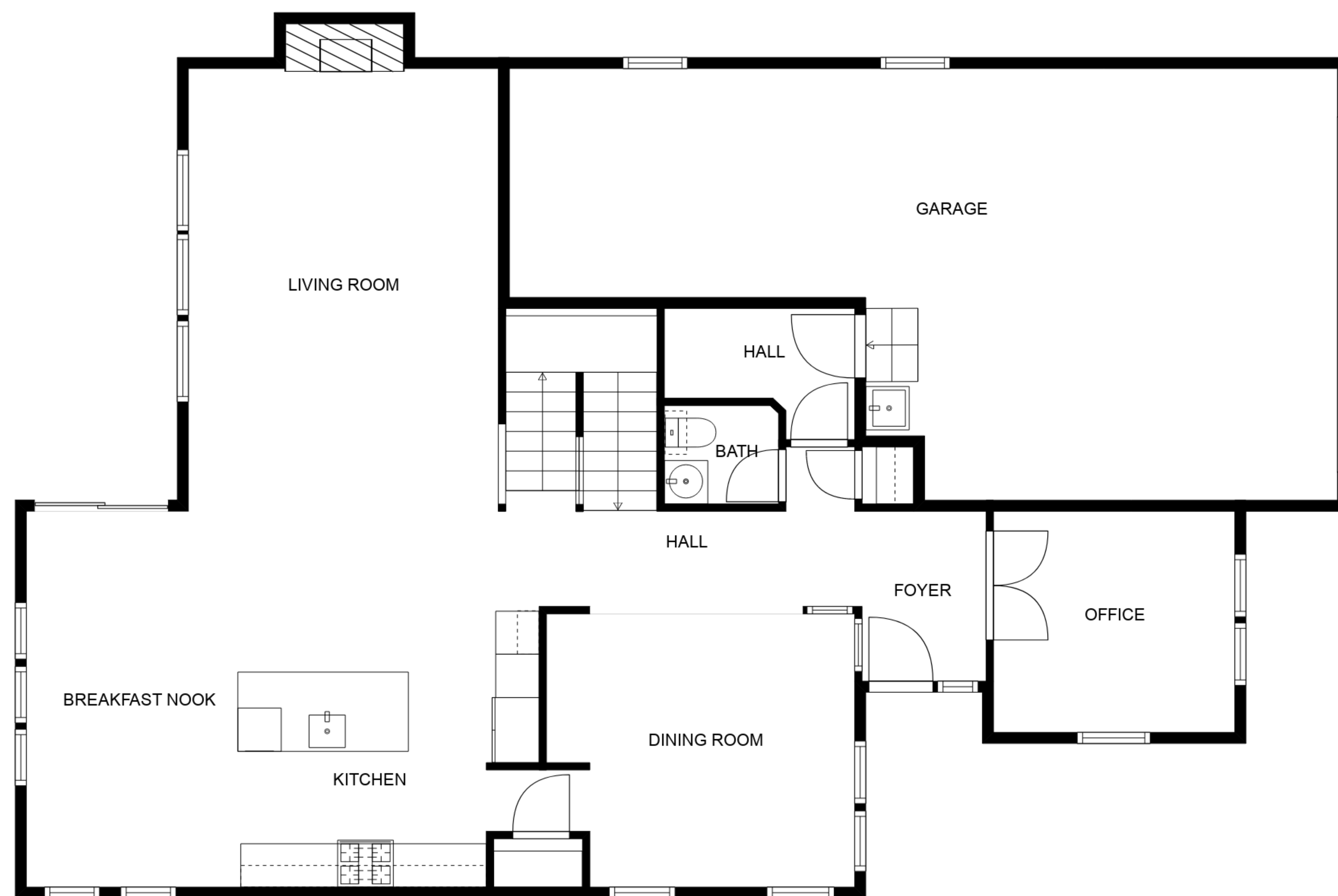
FLOOR 2
