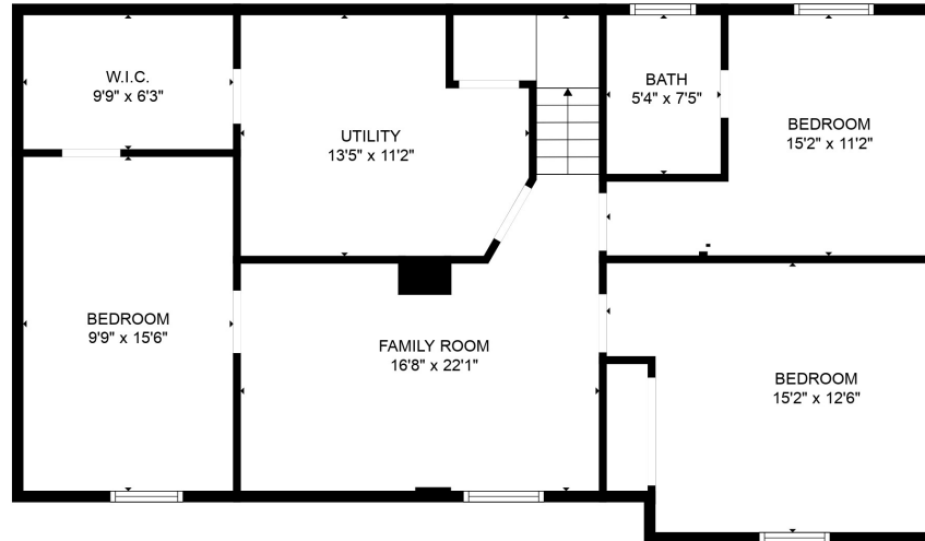
FLOOR 1
