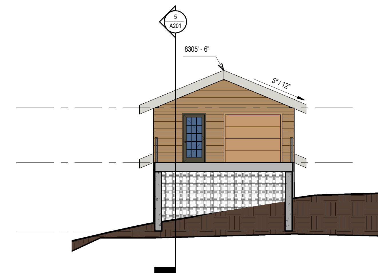
3 WEST ELEVATION 1/8" = 1'-0"
