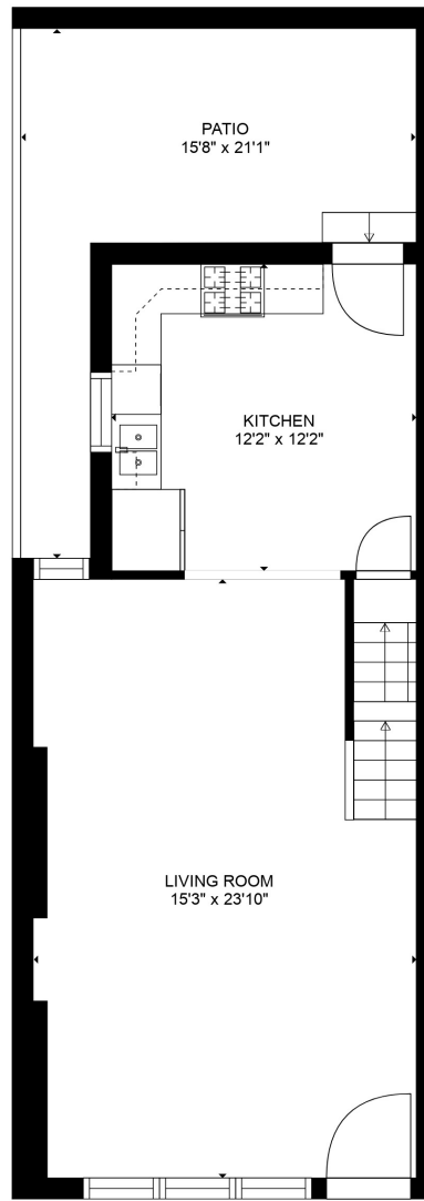
FLOOR 2
