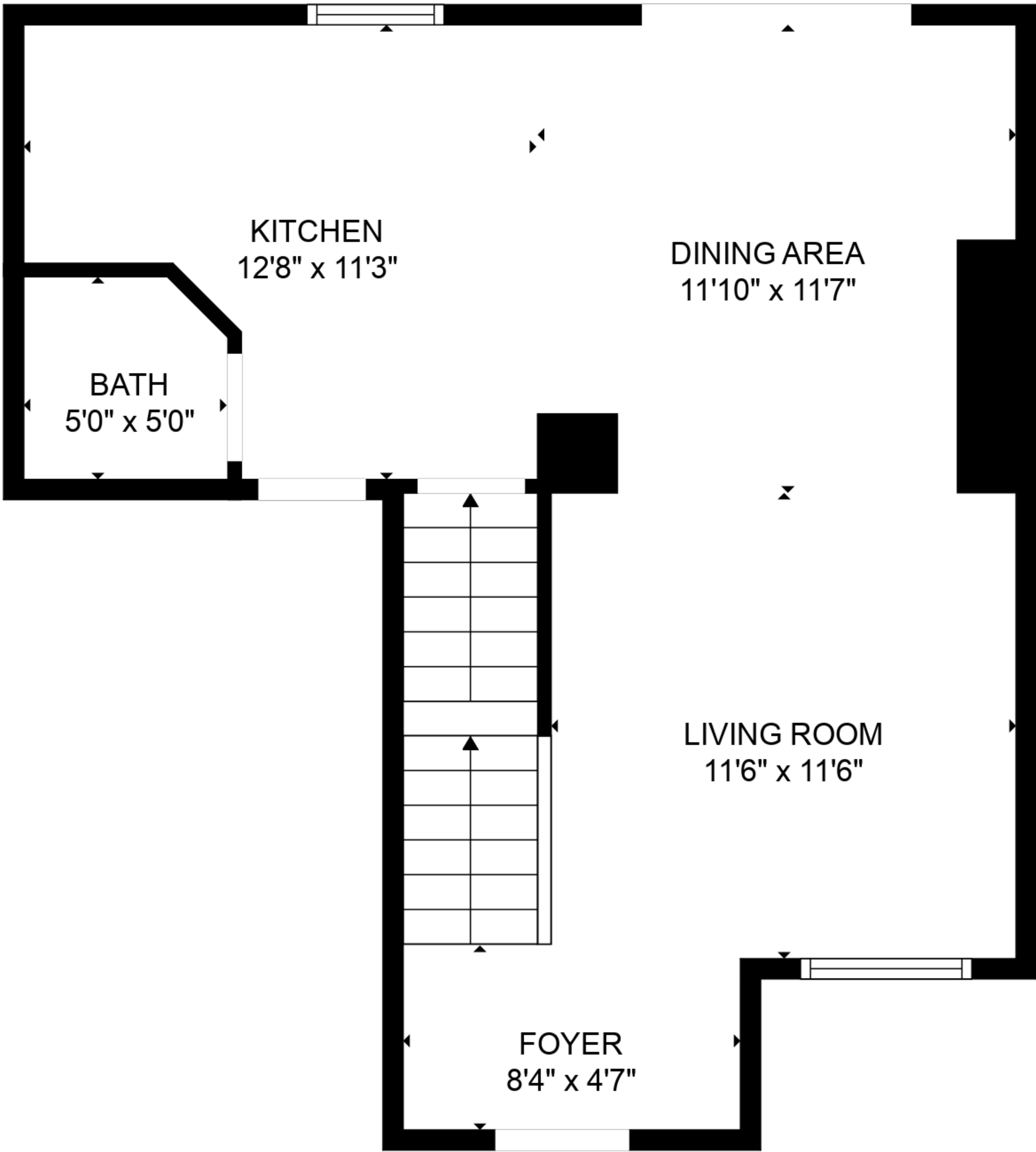
FLOOR 2
