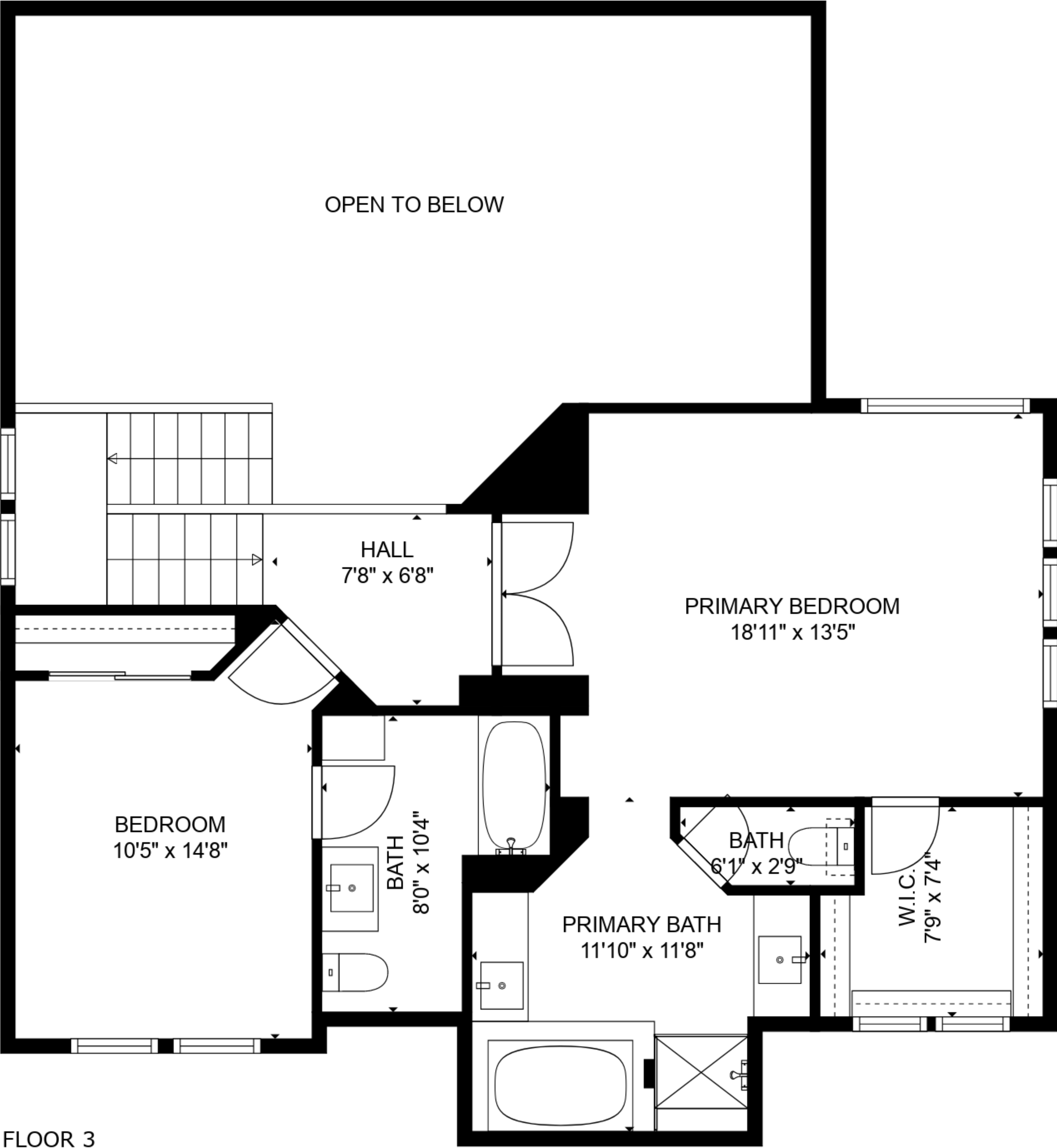
FLOOR 3
