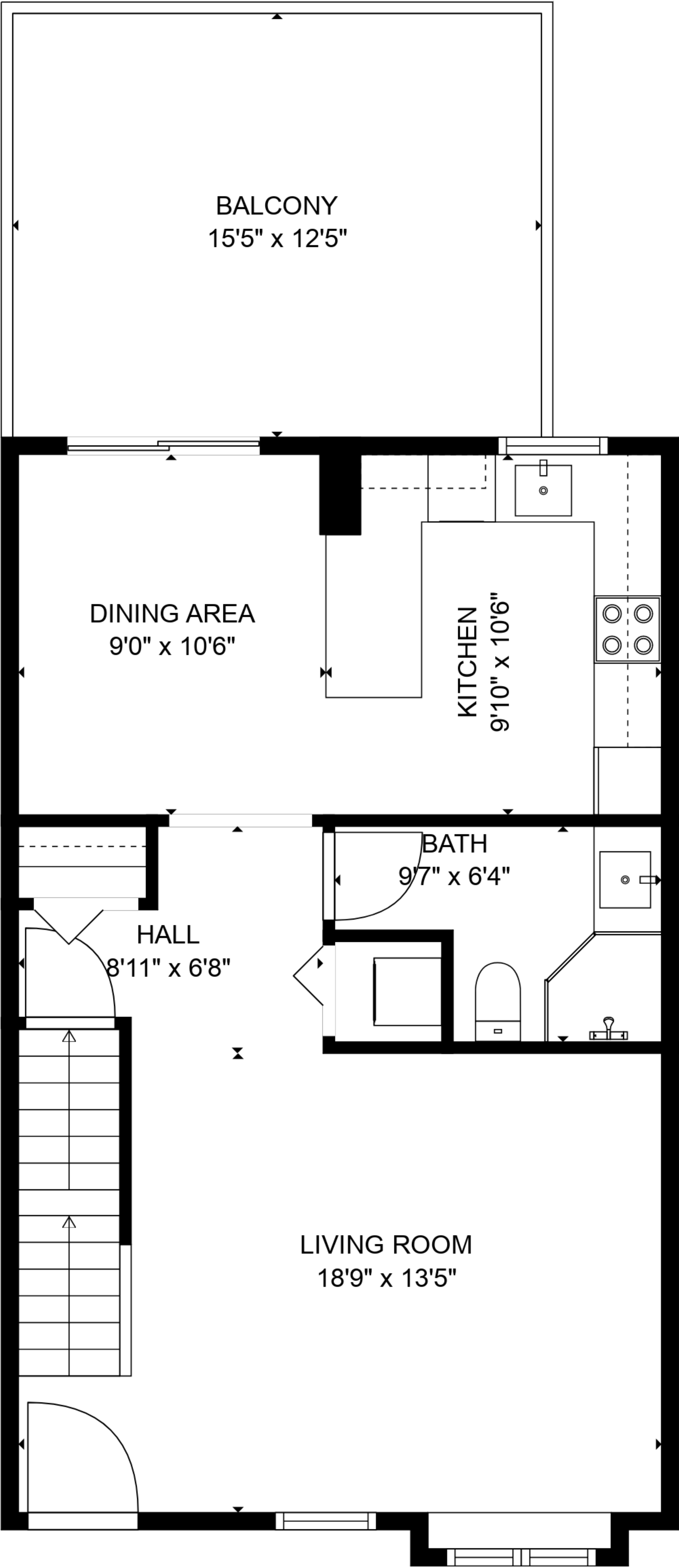
FLOOR 2
