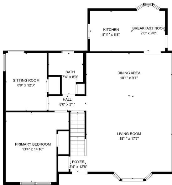
FLOOR 2
