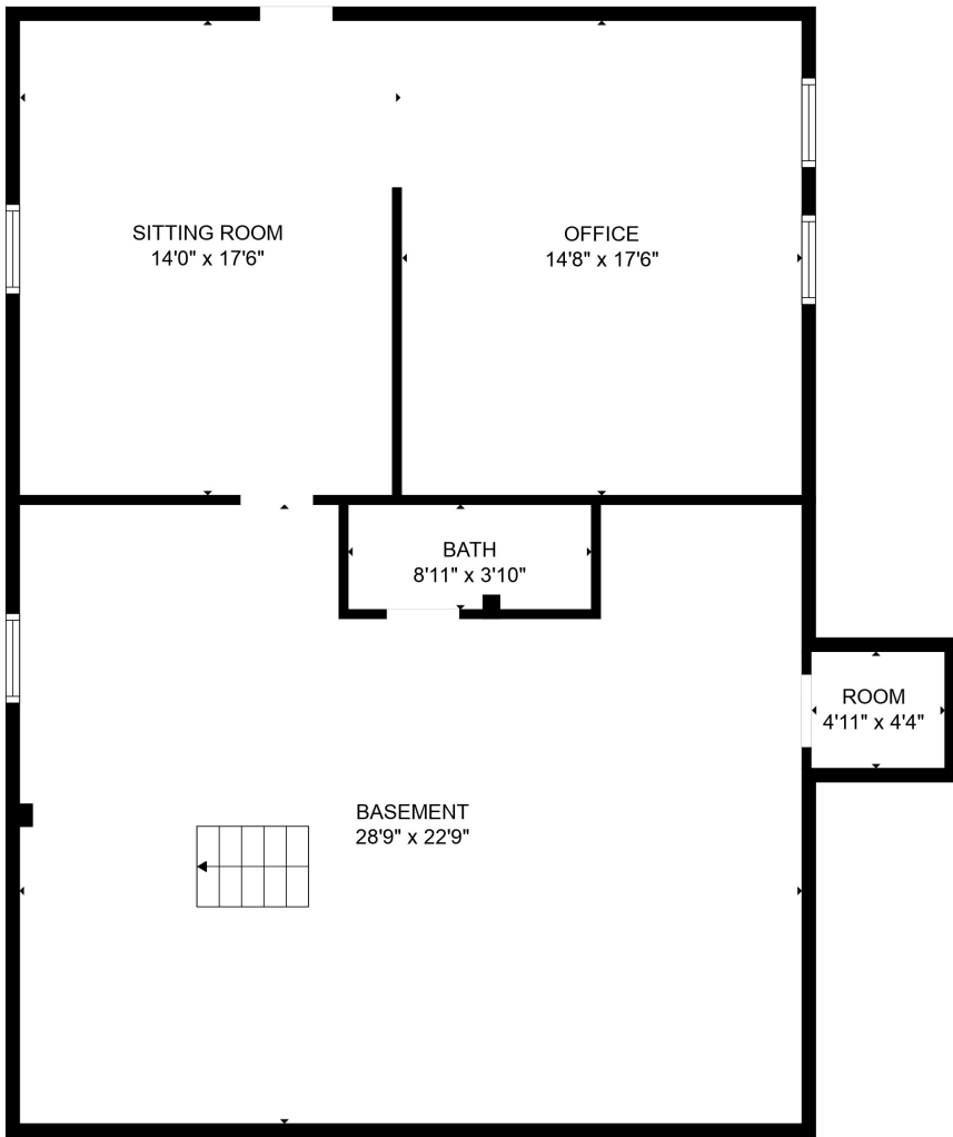
FLOOR 1
