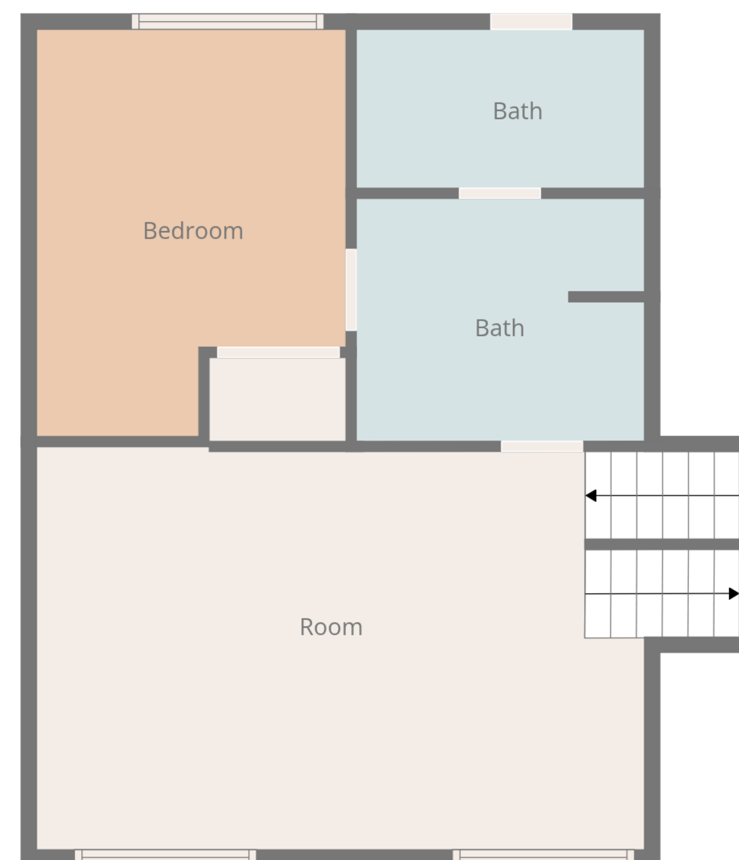
Floor 2
