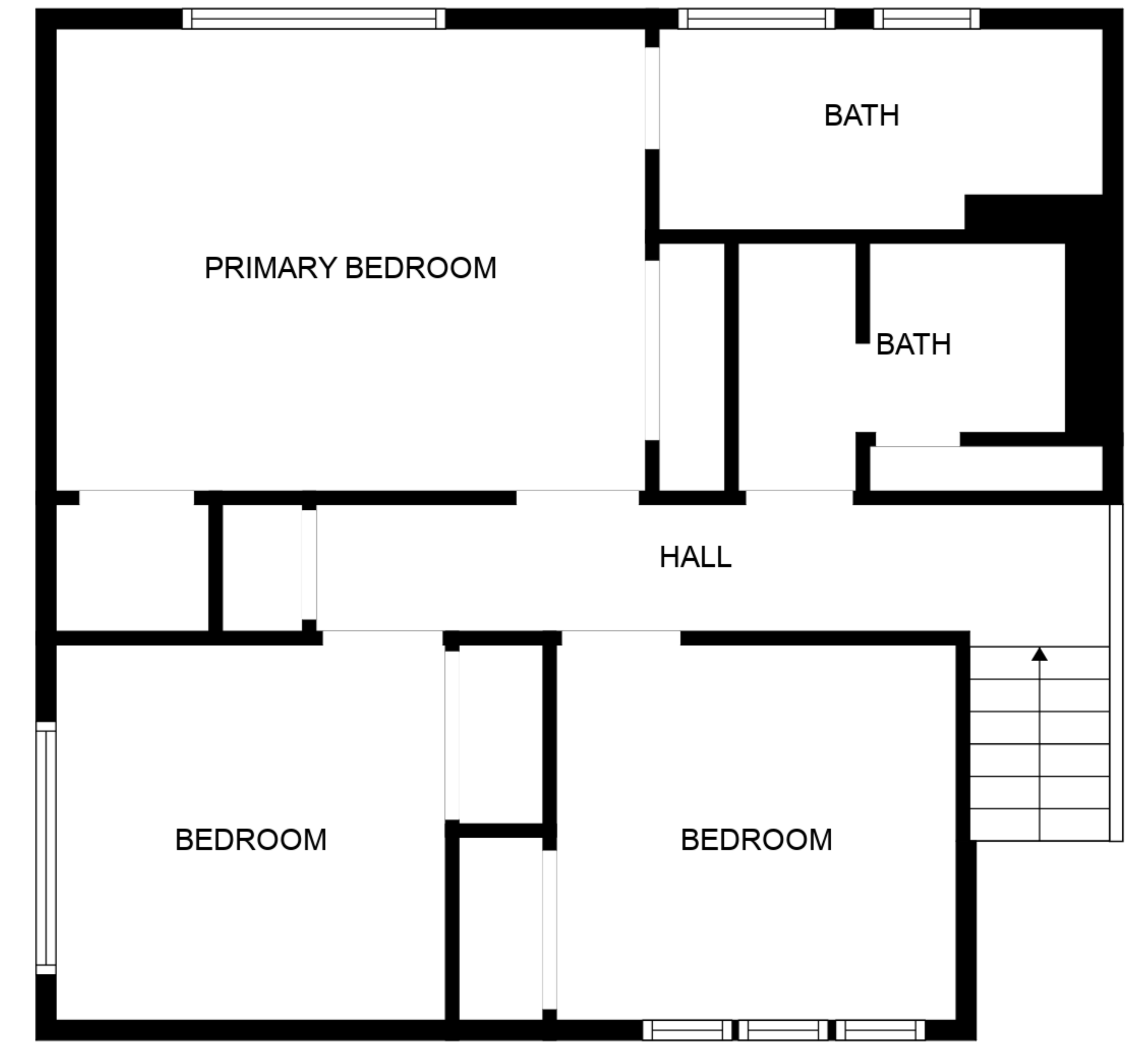
FLOOR 3
