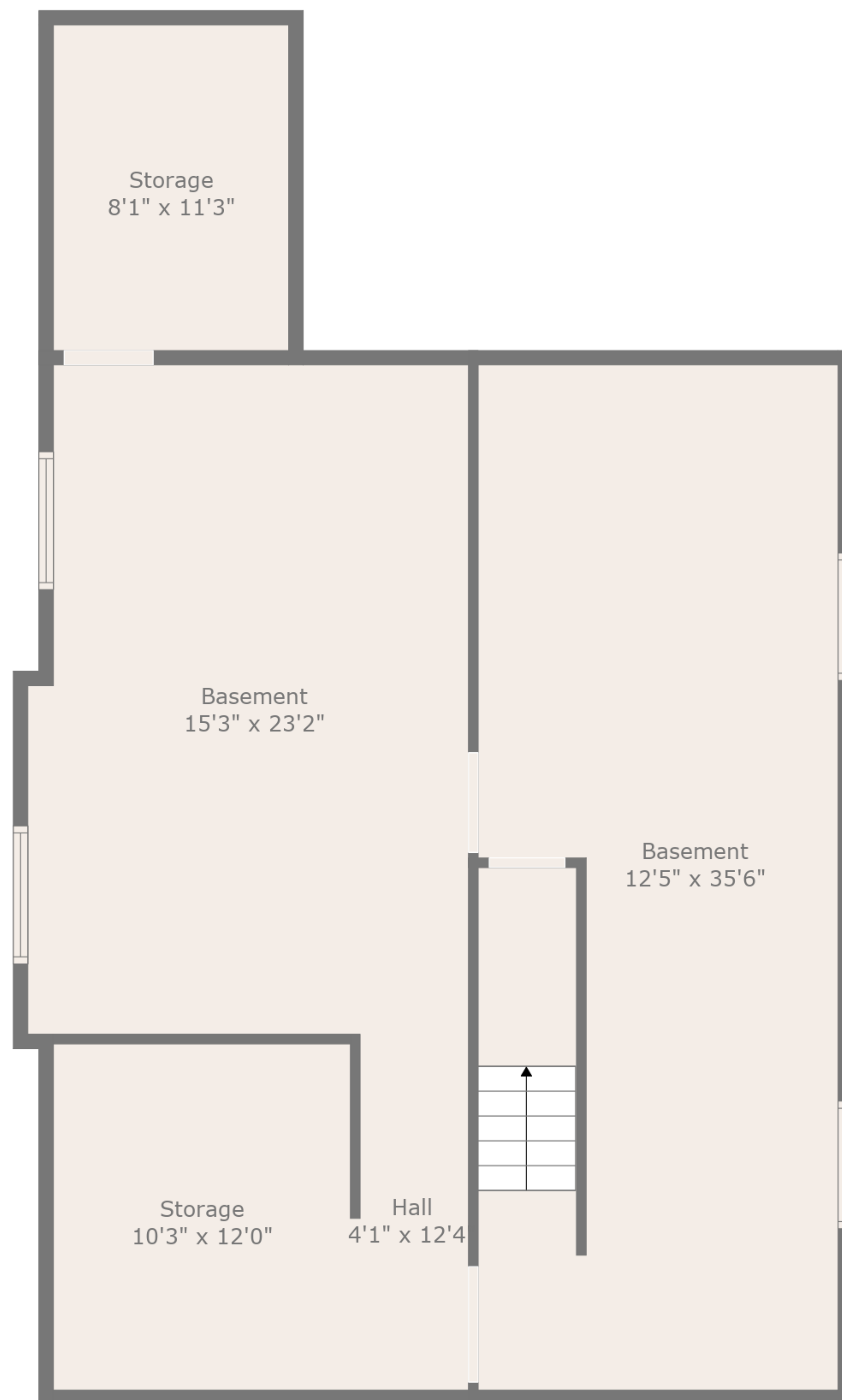
Floor 1
