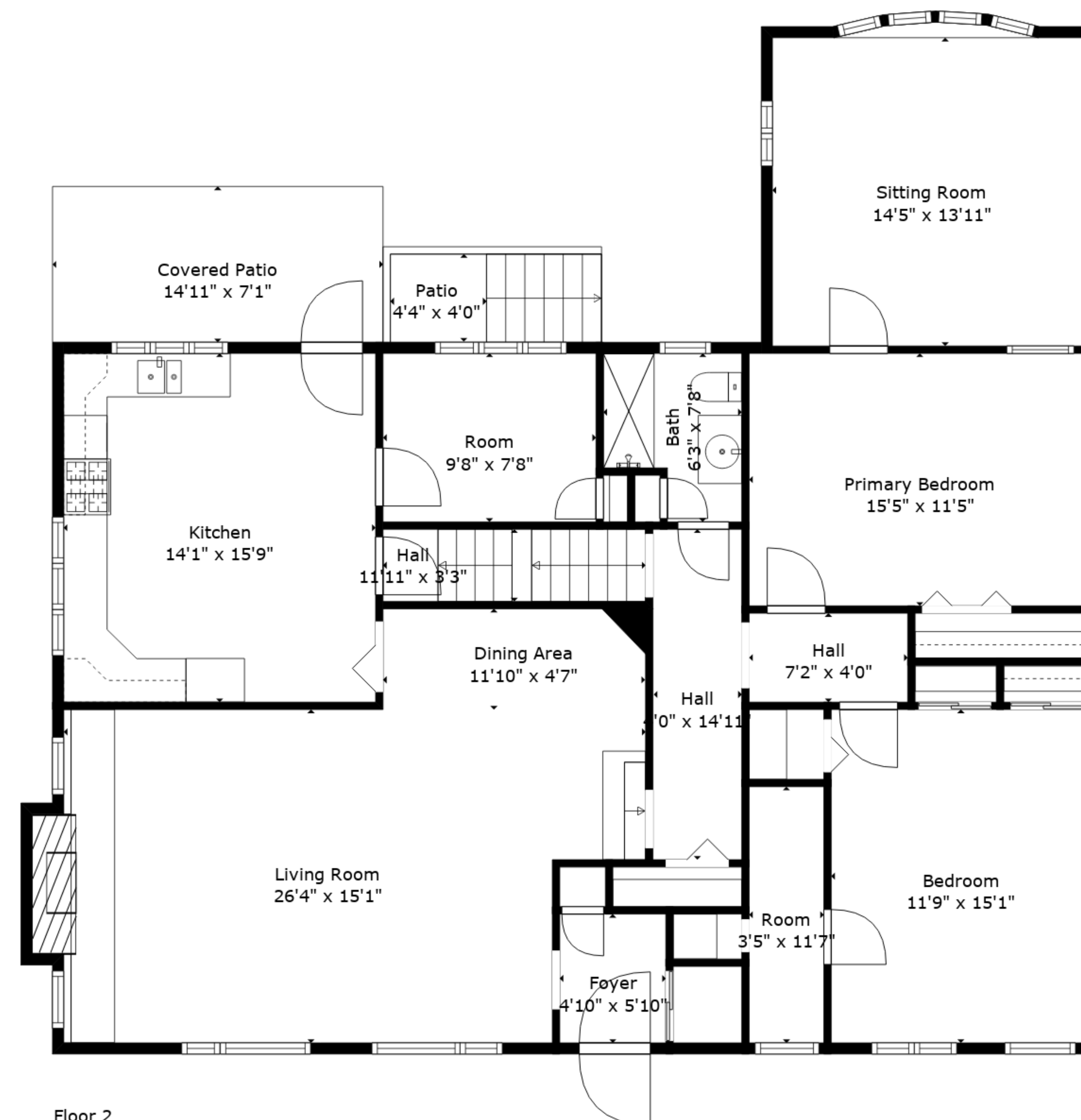
Floor 2
