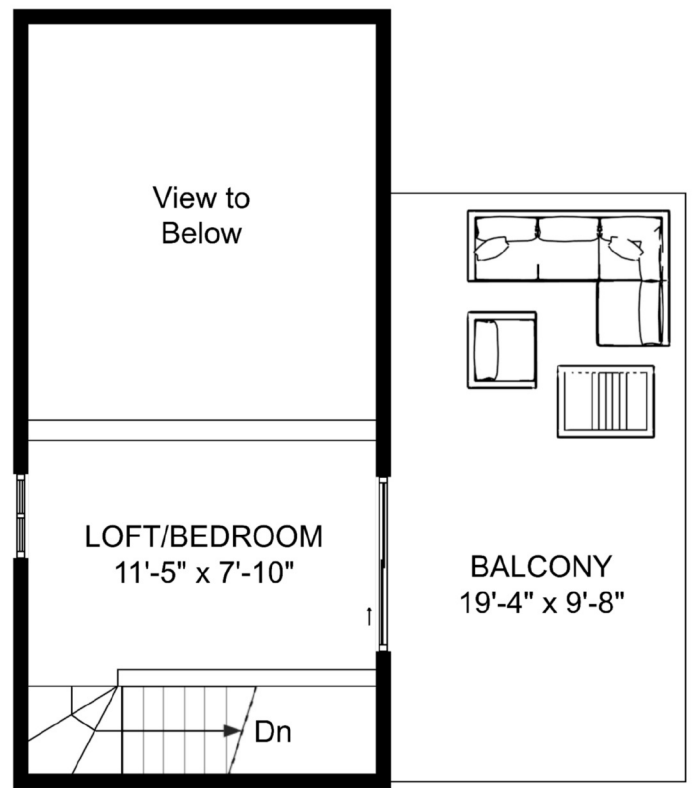
UPPER FLOOR 153 sq.ft. | Ceiling Height: 8'-0"
