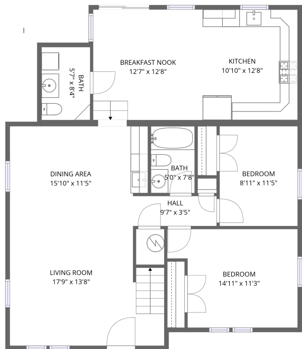
1st floor
