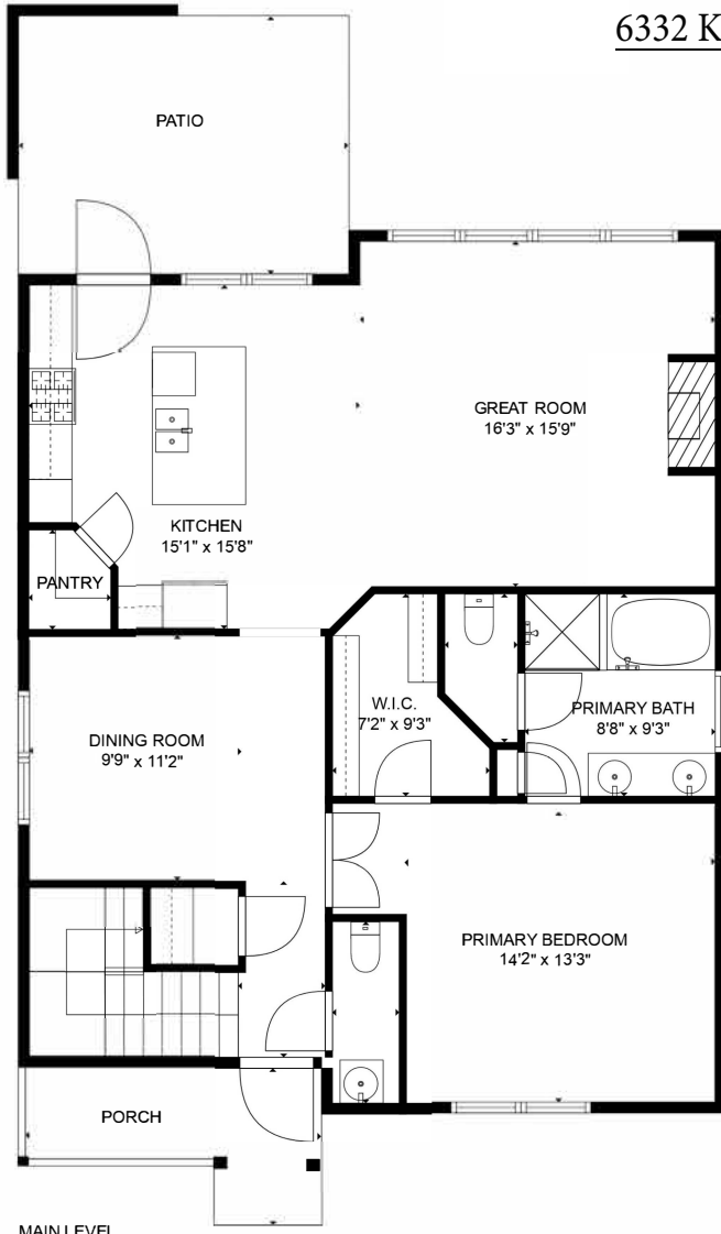
MAIN LEVEL
