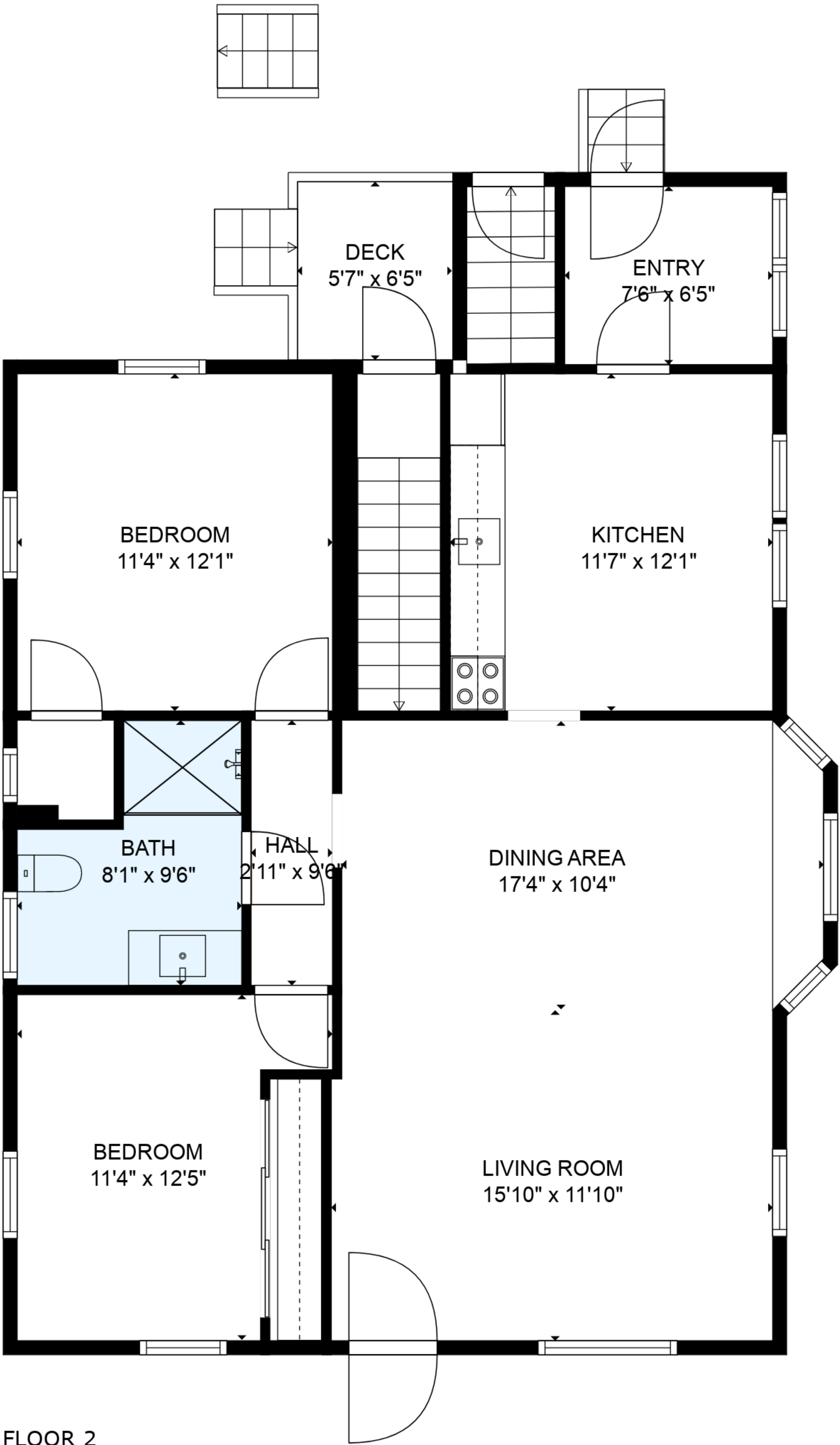
FLOOR 2
