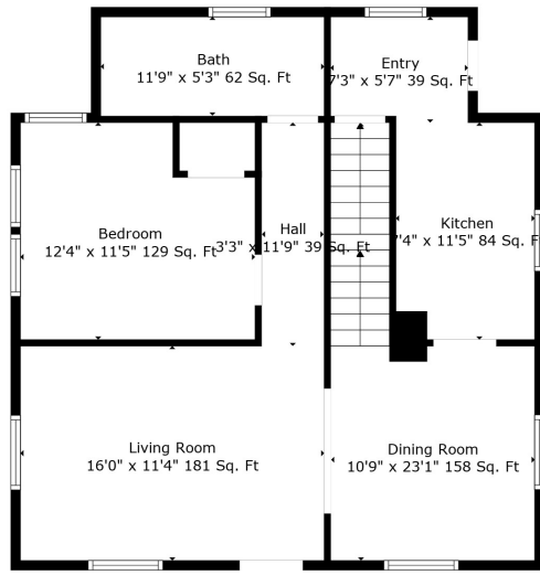
Floor 2
