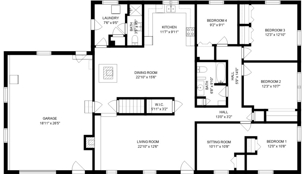
MAIN FLOOR
