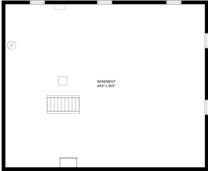
LOWER FLOOR
