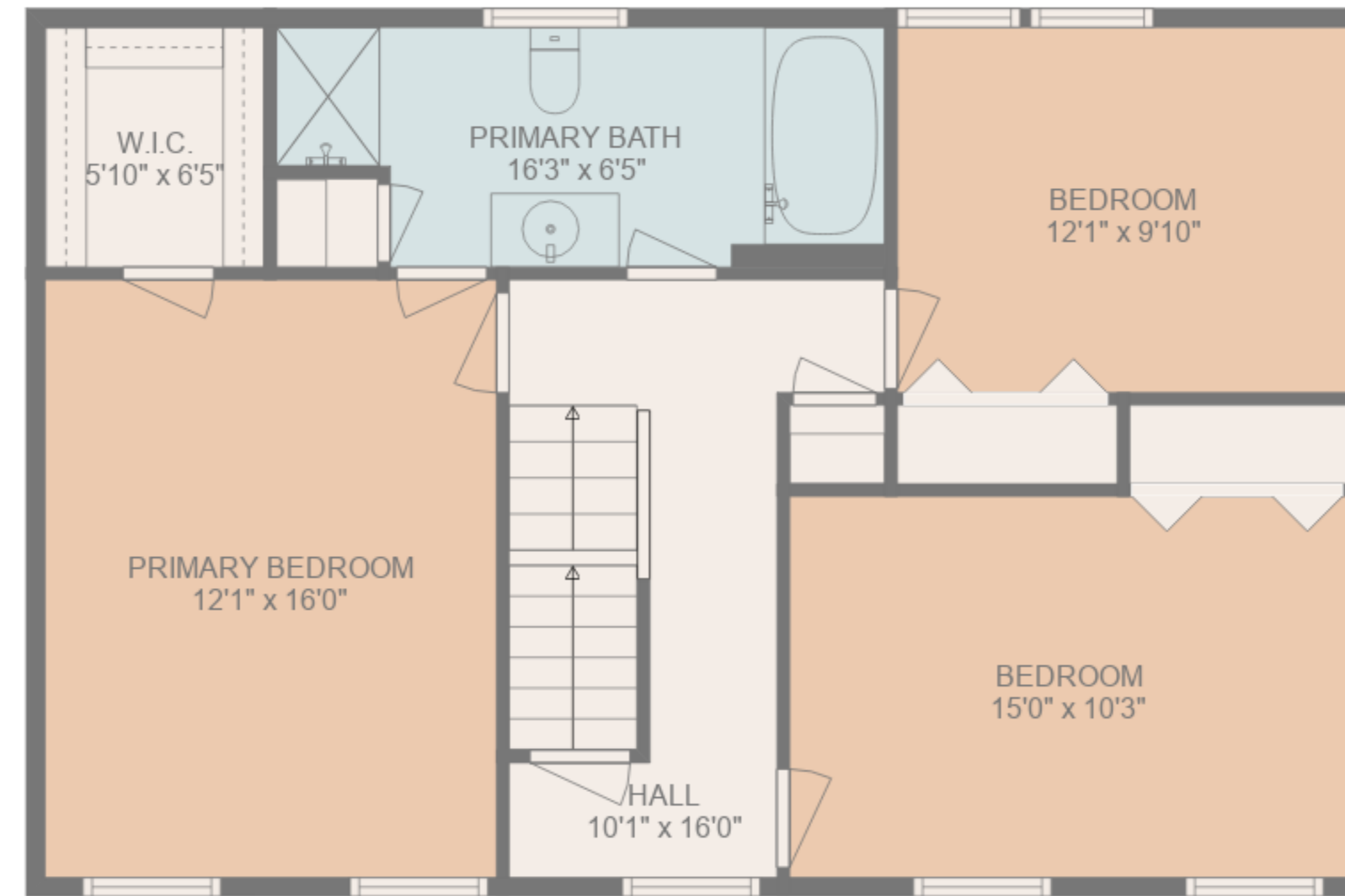
FLOOR 3
