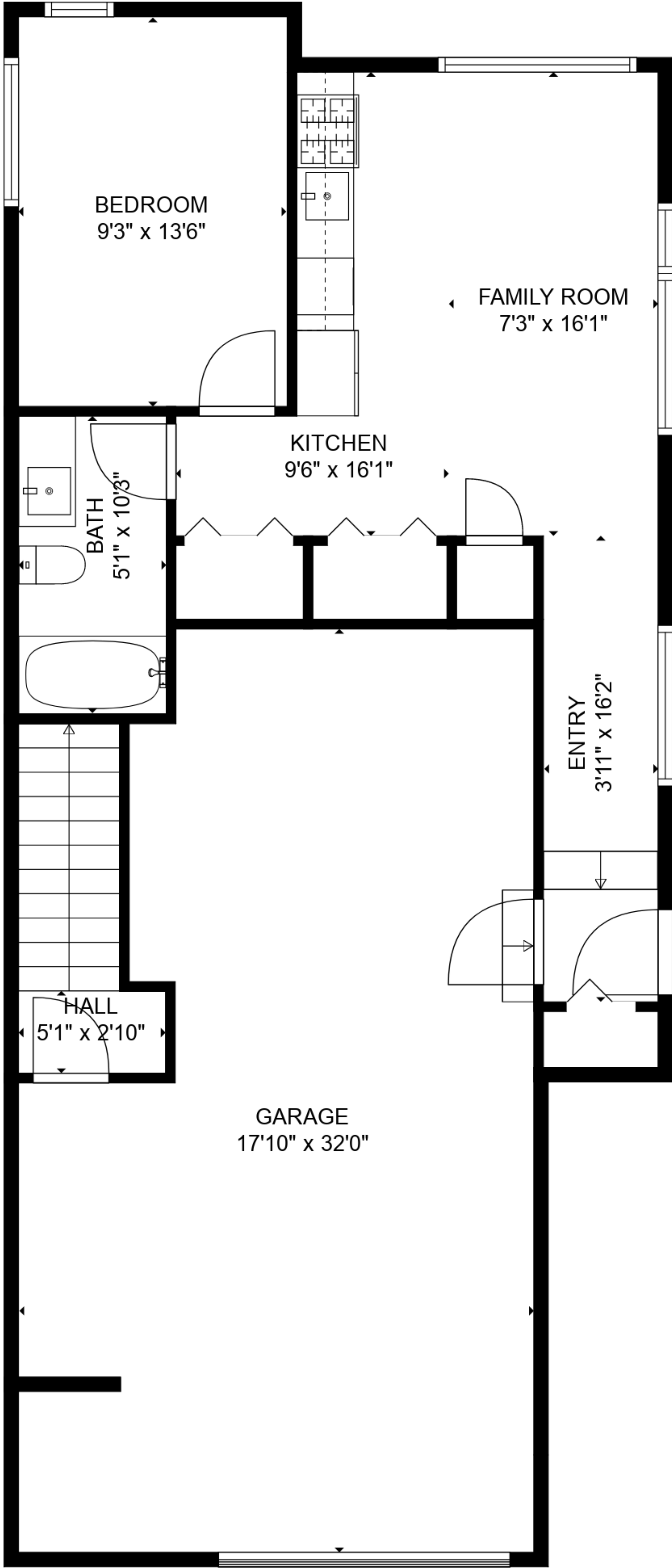
FLOOR 1
