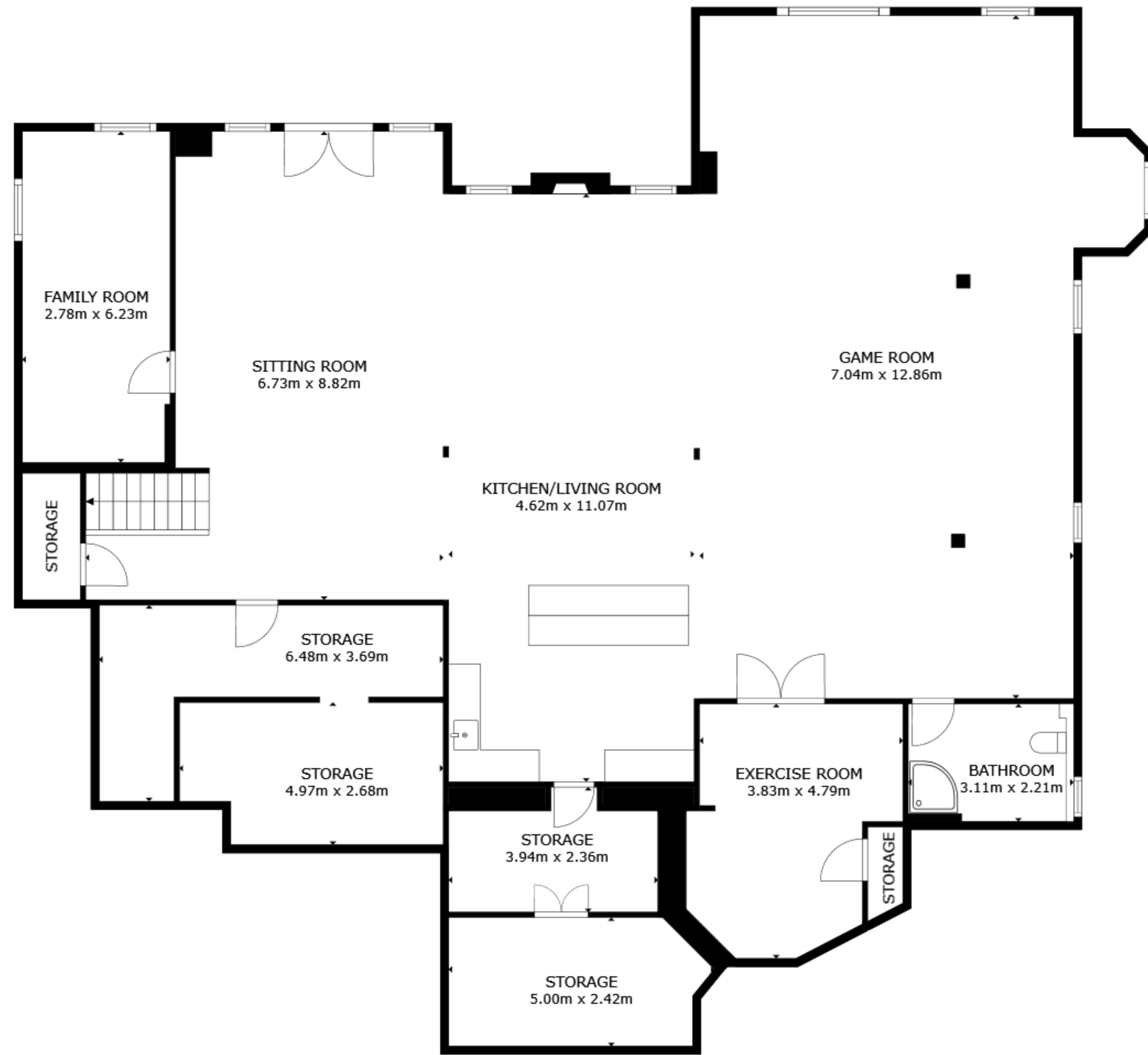
FLOOR 1
