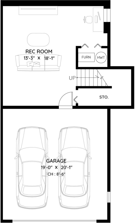
LOWER FLOOR 427 SQ.FT. CH: 8'-0"
