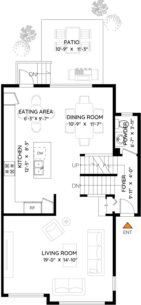
MAIN FLOOR 832 SQ.FT. CH: 9'-0"
