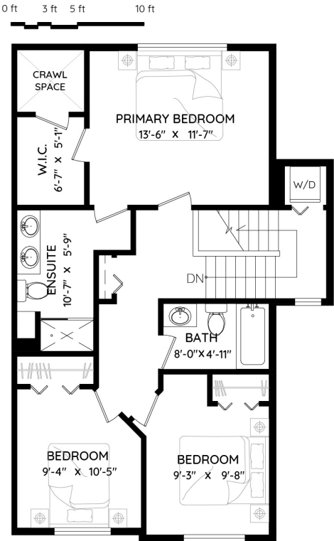
UPPER FLOOR 763 SQ.FT. CH: 8'-0"
