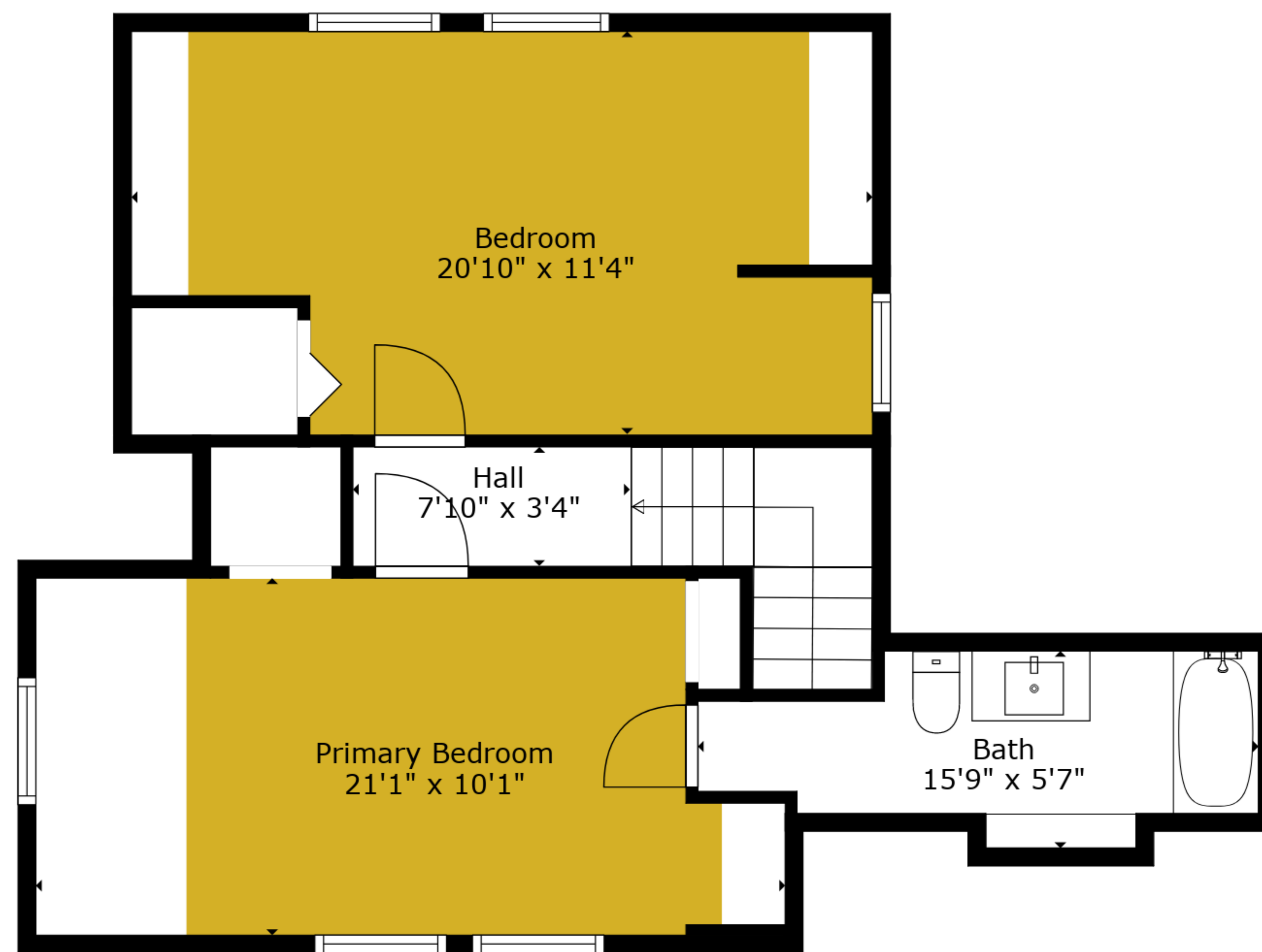
Floor 2
