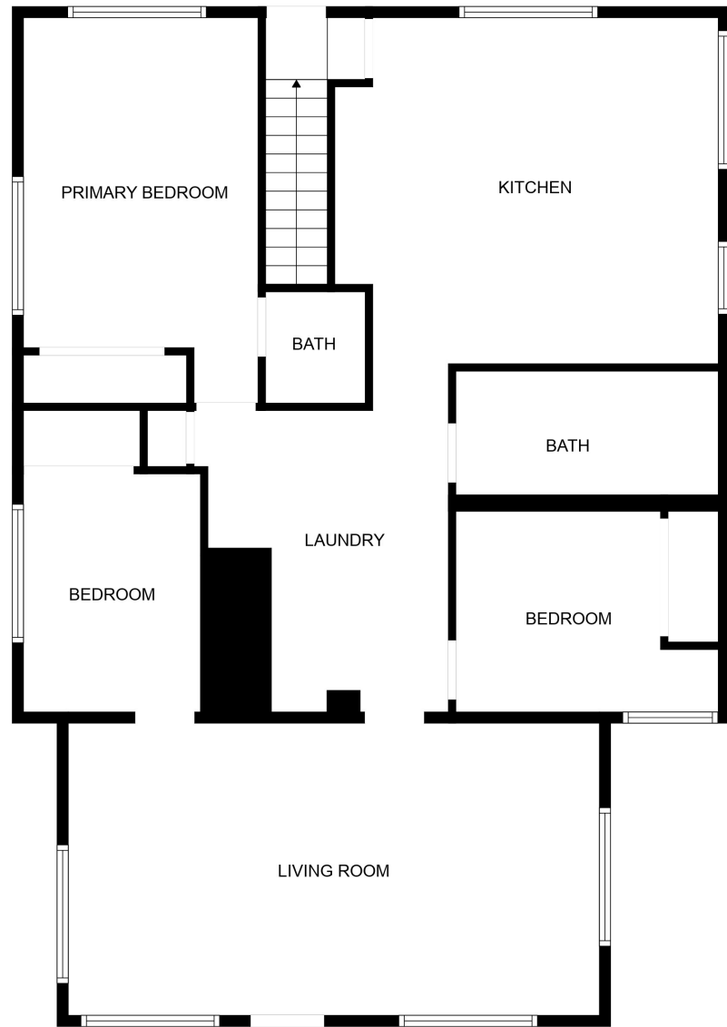
MAIN FLOOR
