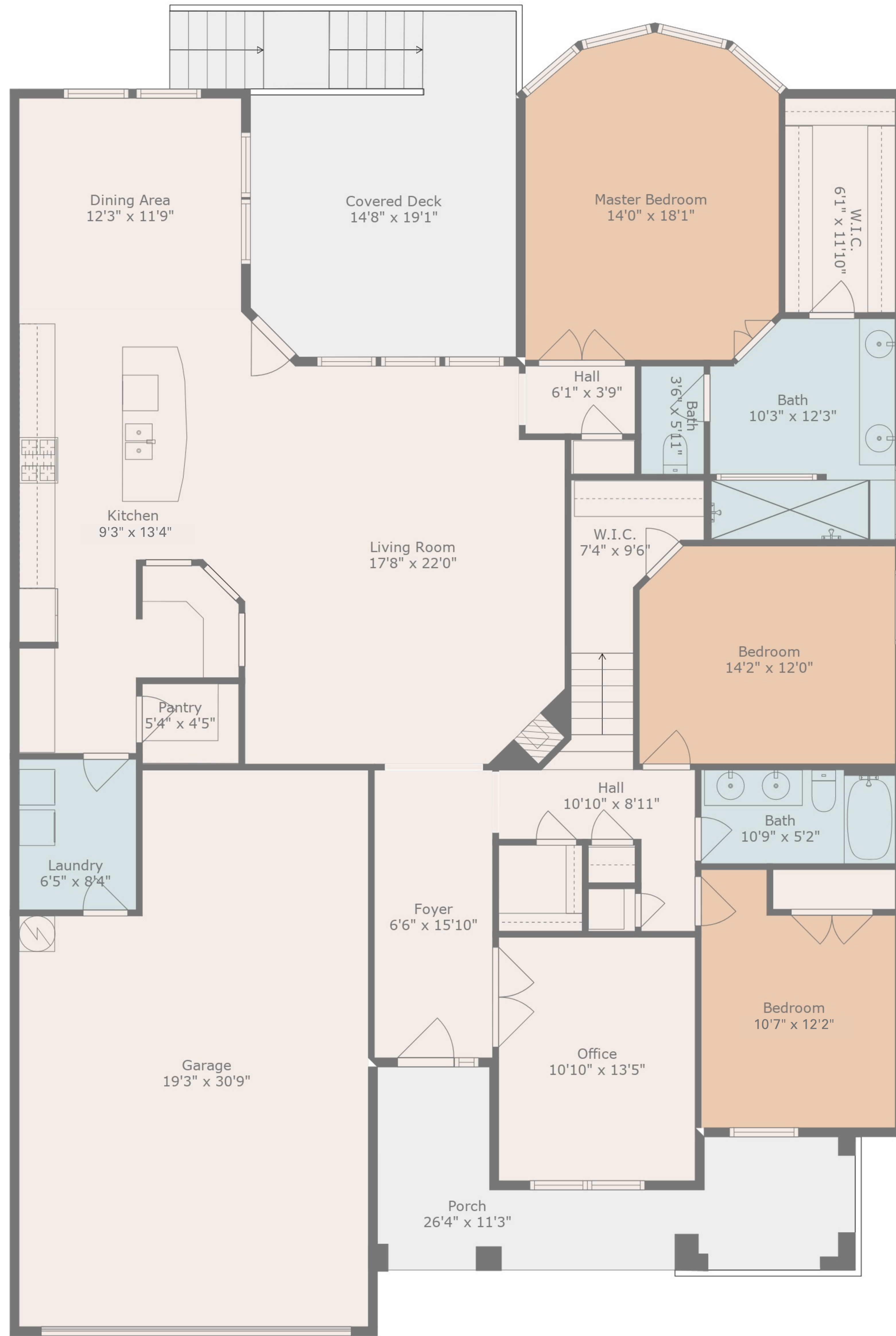
Floor 1
