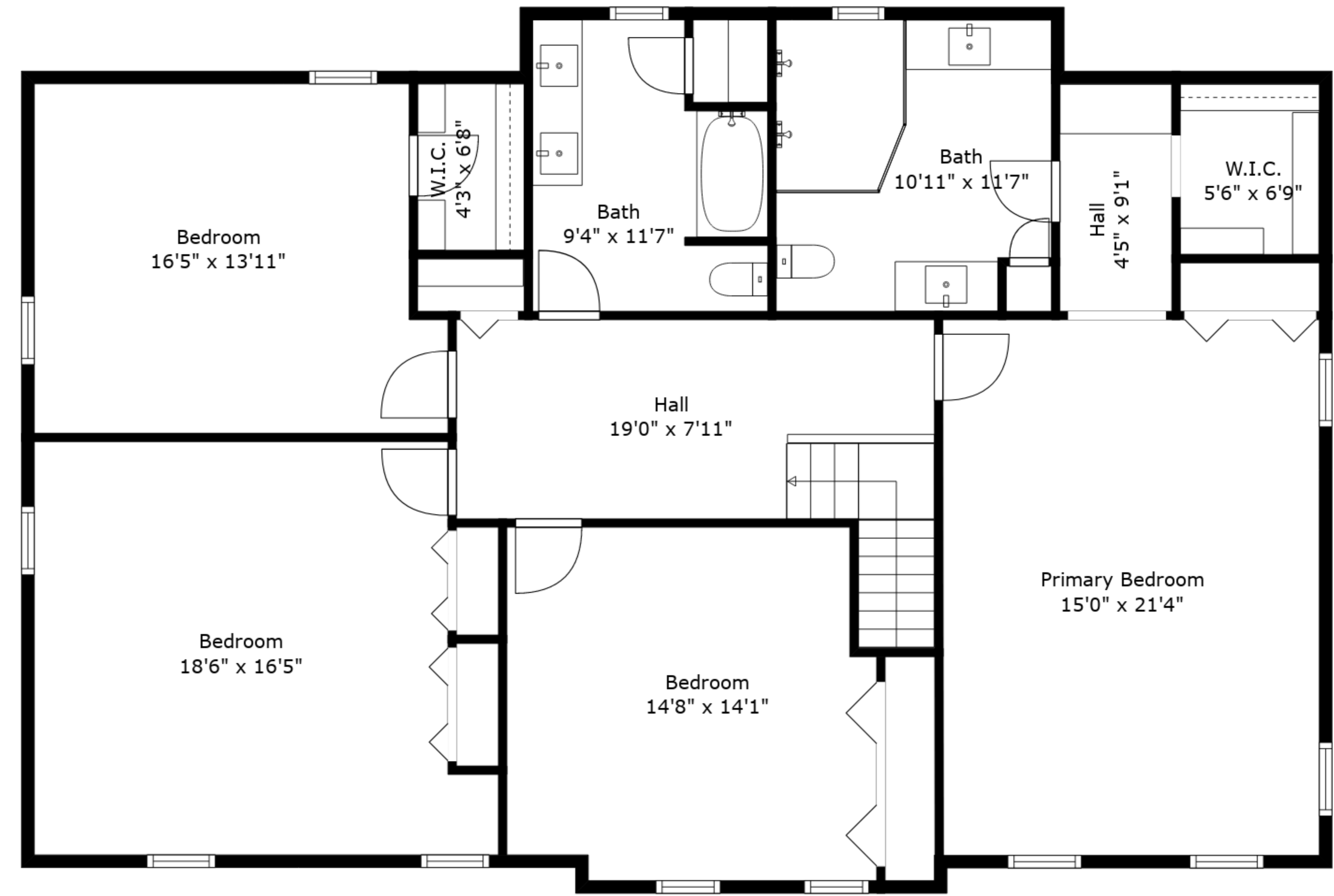
Floor 3
