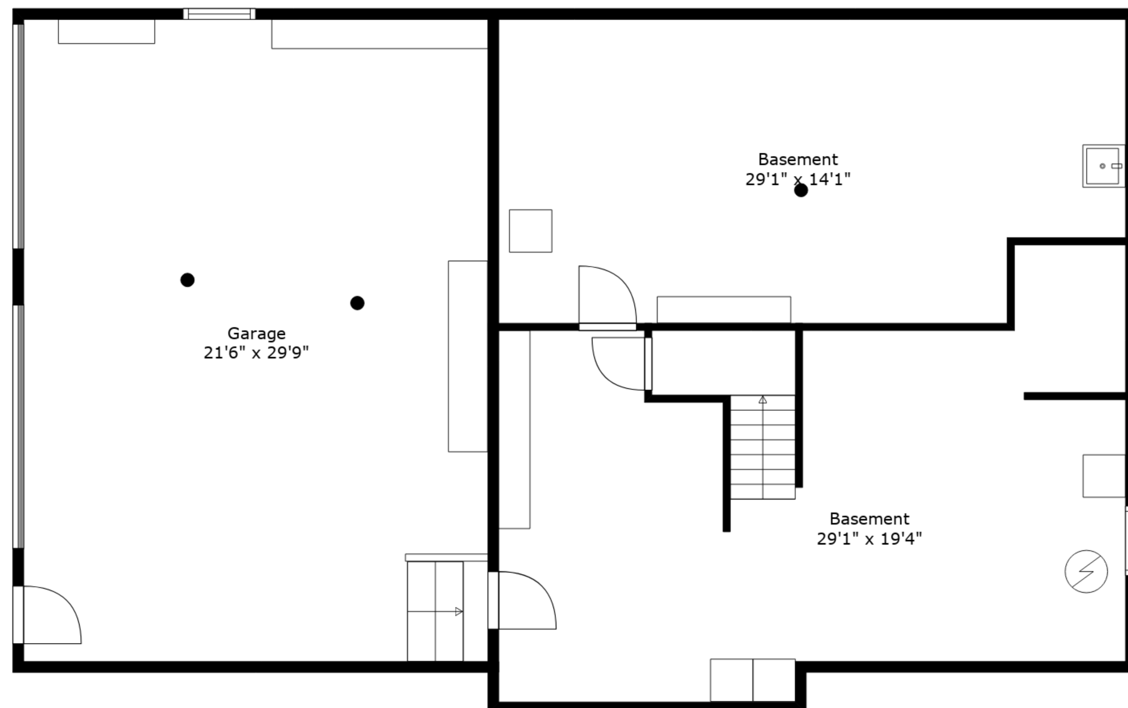
Floor 1
